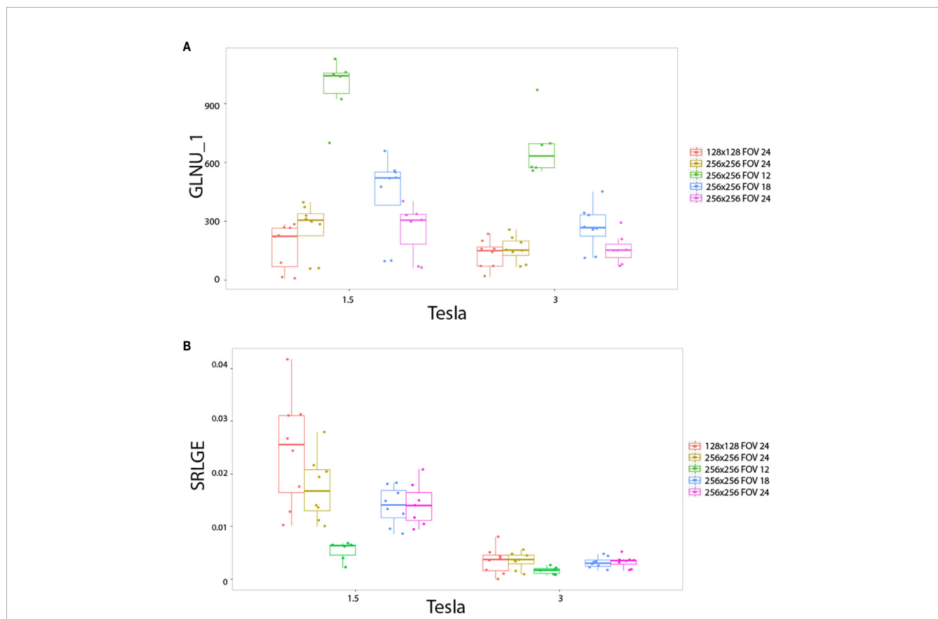
FIGURE 5 | In vitro parameters value according to magnetic field strength and pixel size: for GLNU_1 (A) and SRLGE (B). Texture features extracted to the heterogeneous phantoms. Each colored dot groups and related box plot shows the value of GLNU_1 (A) and SRLGE (B) calculated from repeated phantom MRI acquisition (one dot per MRI acquisition) with different pixel size (one color per matrix/FOV couple), respectively, at 1.5 and 3T.
