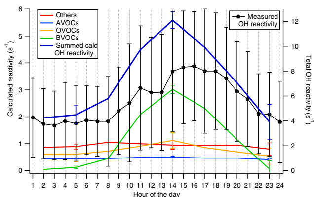
Figure 3. Diurnal patterns of measured (value with \pm 1\sigma , right axis) and calculated OH reactivity (left axis). Others, AVOCs, OVOCs, and BVOCs are the contribution of CO and \text{NO}_x (others), anthropogenic volatiles, oxygenated volatiles and biogenic volatiles to the summed calculated OH reactivity.
