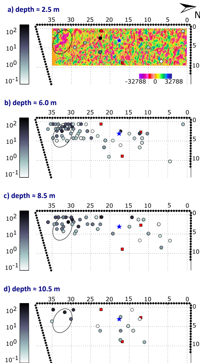
Figure 10. Analysis of the substitution cuttings. The solid circles denote the 1.2-DCB concentrations [ \text{mg}\cdot\text{kg}^{-1} ] measured on the cuttings retrieved. The darker the grey level, the higher the concentration, as indicated by the colorbars next to each map. The initial depths of the cuttings are comprised between 2.0 m and 2.9 m for (a), between 5.3 m and 6.3 m for (b), between 7.9 m and 9.4 m for (c), between 9.8 m and 11.0 m for (d). The map of the GPR amplitudes obtained at 1.3 m depth is superimposed on the plot corresponding to the closest depth (Figure 10a). The black oval locates the GPR anomalous reflector. The small black dots outside of the surveyed area represent the reinforced concrete piles. The blue star denotes the former piezometer P57 and the red squares the former sparging heads.
