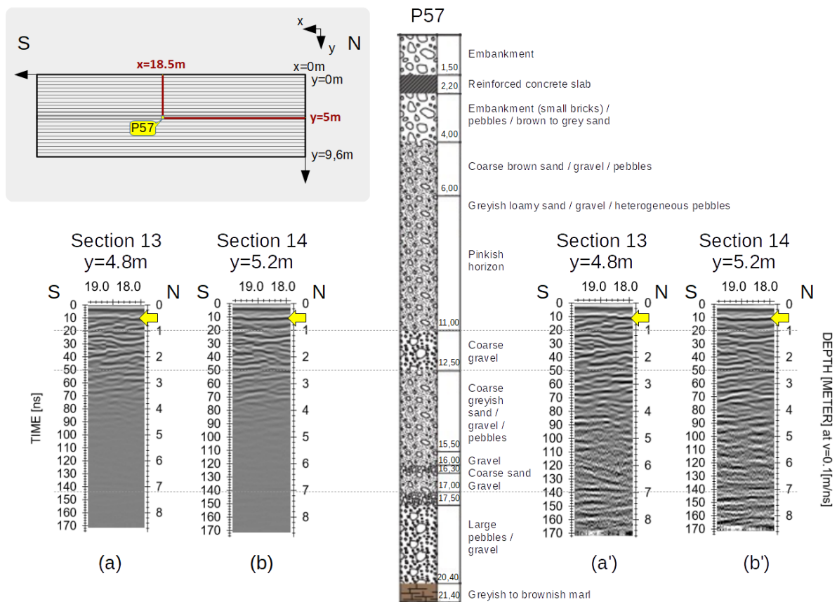
Figure 5. Correlation between radargrams acquired at y = 4.8\text{ m} (a) and y = 5.2\text{ m} (b) between x = 18\text{ m} and y = 20\text{ m} and the lithological log at borehole P57. The same radargrams were represented with a different gain (energy decay) in (a') and (b'). The yellow arrows designate the WT.
