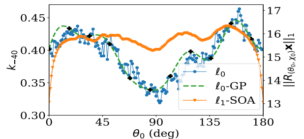
Fig. 4. Effective sparsity k_{-40} for \chi_0 = 0^\circ , containing the lowest sparsity on the research domain, its GP estimation and the \ell_1 norm found by the SOA method of the spherical coefficients for the 12 GHz reflectarray measurement. The GP curve is derived from the discrete set of values represented by black markers. The \ell_1 only reaches a local minimum.
