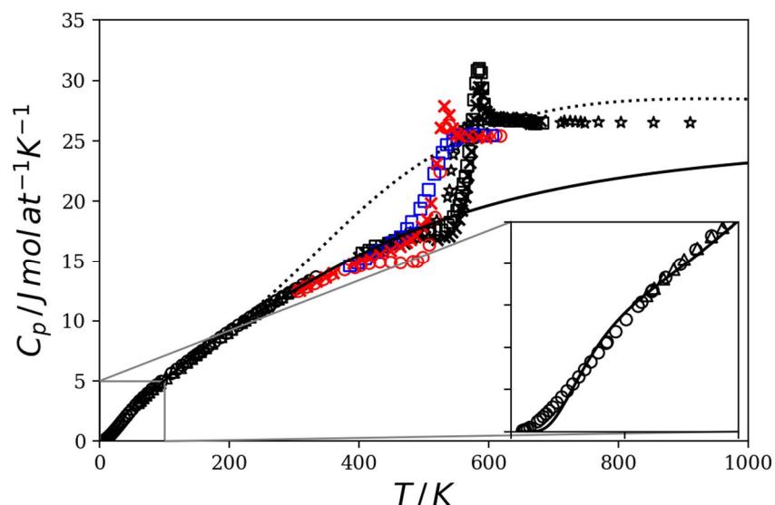
Figure 3. Heat capacity of B_2O_3 at the glass and liquid states. Adiabatic calorimetry: black ( \Delta ) Turdakin and Tarasov [62], black ( \circ ) Richet et al. [63], black ( \star ) Shmidt [60]. Radiation scanning calorimetry: red ( \circ ) on heating after very fast cooling, blue ( \square ) on cooling from the liquid, red ( \times ) on heating after slow cooling, Thomas and Parks [64]. DSC: black ( \square ) on heating at 10 \text{ K min}^{-1} after prior cooling at -10 \text{ K min}^{-1} , black ( \times ) on heating at 10 \text{ K min}^{-1} after prior cooling at -80 \text{ K min}^{-1} Moynihan et al. [65]. Modeling from this work, solid-like state (solid line), liquid (dotted line).
