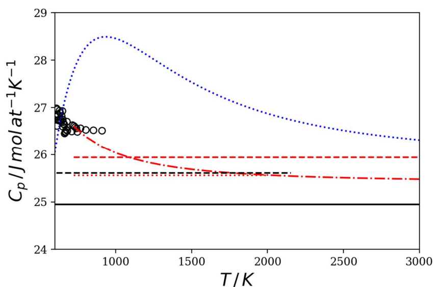
Figure 5. Heat capacity of equilibrium B_2O_3 liquid. Horizontal solid line = 3R Dulong-Petit limit. ( \circ ) selected measurements from Shmidt [60] by adiabatic calorimetry or Moynihan et al. [65] by DSC. Black dashed line, constant 25.611 \pm 0.064 \text{ J mol at}^{-1} \text{ K}^{-1} heat capacity from linear regression to heat increment measurements. Red
