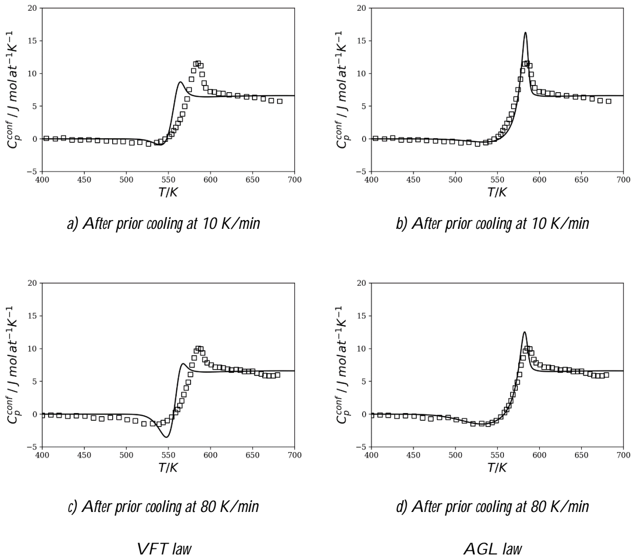
Figure 11. Liquid configurational heat capacity vs. temperature in the glass transition range on heating at 10 K/min. ( \square ) Experimental points from Moynihan et al. [65]. Black curve = modeling from this work with the recommended values of the liquid two-state model A, B parameters given in Table 6.
