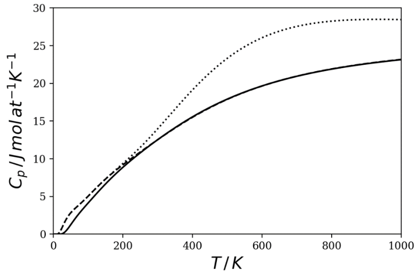
Figure 7. B_2O_3 heat capacity curves for the crystal (solid line), the "sol" phase (dashed line) and the equilibrium liquid (dotted line) phases calculated from this work with the coefficients given in Tables 3, 4 and 6.
