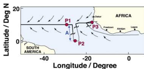
Figure 1. The cruise track is shown. Black arrows indicate the prevailing trade winds and the tildes indicate where the ITCZ was crossed. The letter A marks the north south section shown in Figure 3. P1 to P3 mark the positions of depth profiles plotted in Figure 4.
