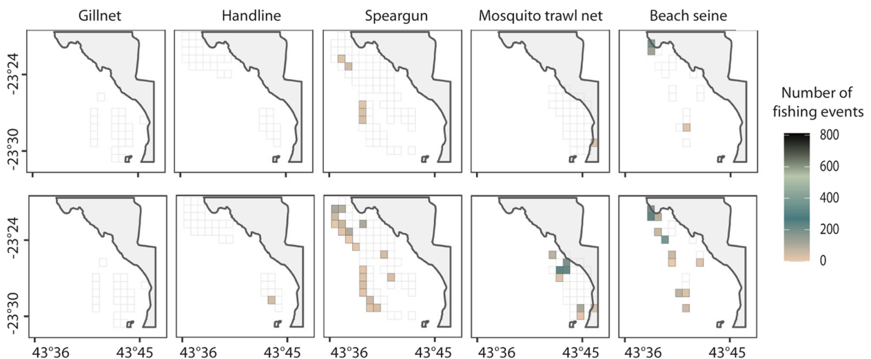
Fig. 3. Maps of spatial sensitivity of the random forest model (A) and the speed threshold method (B) for each gear type using a 0.005^\circ \times 0.005^\circ ( 555\text{ m} \times 555\text{ m} ) cell grid. Only cells with sensitivity < 80\% are coloured for better clarity (see Section 2 for details). The colour gradient shows the difference in the number of fishing events between the observer's measurements and the true positives predicted by both methods. (For interpretation of the references to colour in this figure legend, the reader is referred to the web version of this article.)
