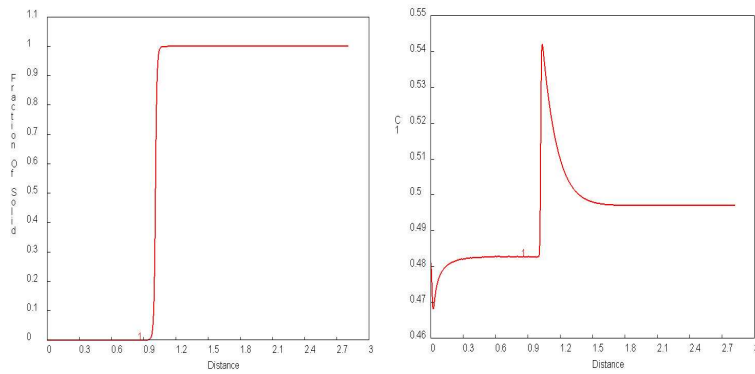
Figure 1: \phi(x) and c(x) at final time for a Ni-Cu alloy
