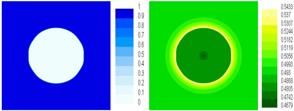
Figure 1: \phi(x) and c(x) at final time for a Ni-Cu alloy
