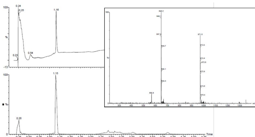
Figure S7: LC-MS traces of 1
