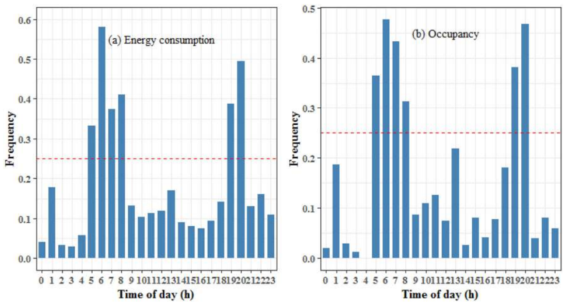
Fig. 5. Results of CPA for energy consumption and occupancy (apartment 1).
