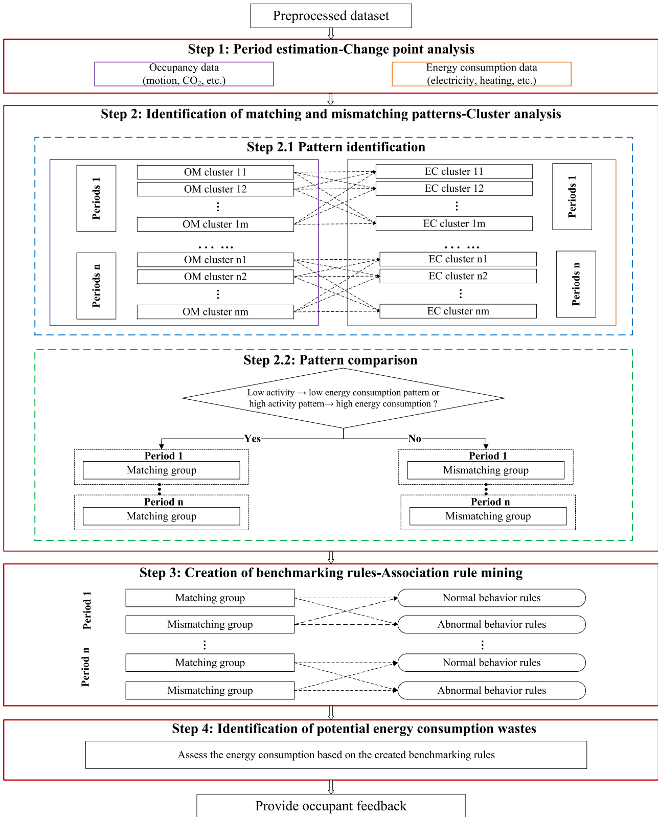
Fig. 1. Framework of the proposed methodology to identify energy waste patterns in residential buildings (EC and OM are the abbreviations of energy consumption and occupant movement).
