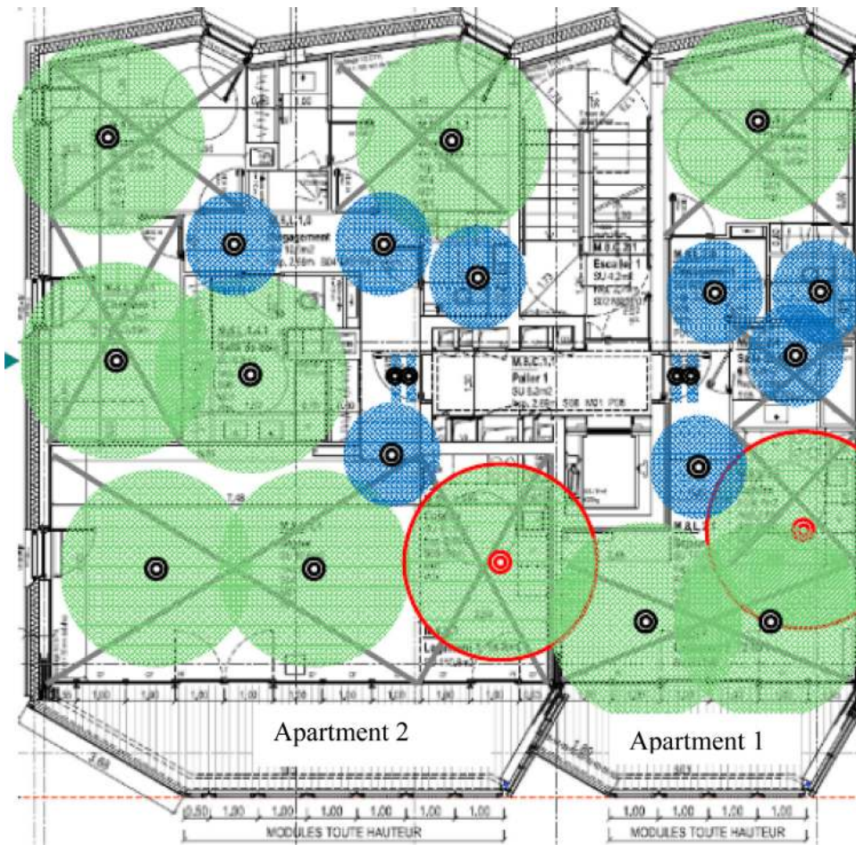
Fig. 4. Floor plan and motion sensors deployed in apartment 1 and apartment 2.
