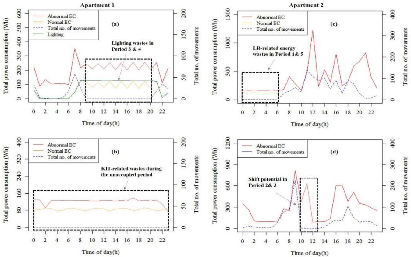
Fig. 13. Illustration of different types of energy waste patterns during a sleeping/away pattern event in apartment 1 & 2.
