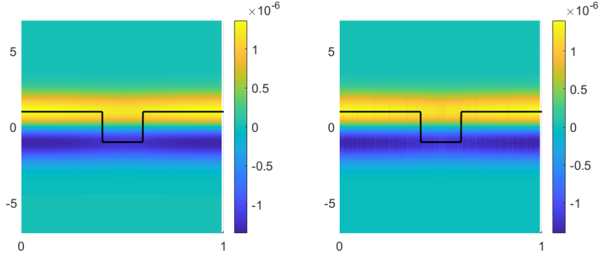
Figure 5: Left: E^\varepsilon(x, y) = n^\varepsilon(x, y) - n^0(y) , where n^\varepsilon(x, y) is determined numerically. Right: theoretical \varepsilon \bar{D}(x, y) . In black, the 1-periodic function \theta given by (152) with a = 0.8 . Here A = 0.9 and \varepsilon = 10^{-4} .
