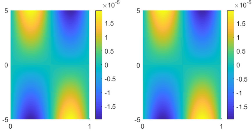
Figure 3: Left: relative error \frac{n^\varepsilon(x,y)-n^0(y)}{n^0(y)} , where n^\varepsilon(x,y) is determined numerically. Right: theoretical relative error \frac{\varepsilon\bar{D}(x,y)}{n^0(y)} . Here A = 0.9 , \varepsilon = 10^{-4} and \theta(x) = \sin(2\pi x) , i.e. L = 1 .
