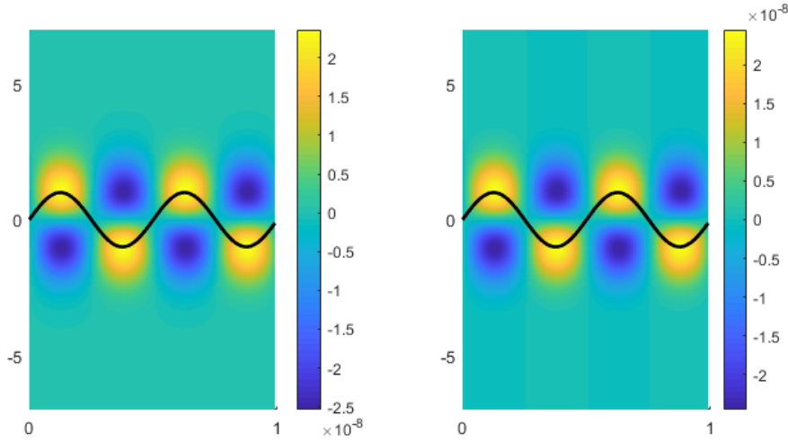
Figure 2: Left: absolute error E^\varepsilon(x, y) = n^\varepsilon(x, y) - n^0(y) , where n^\varepsilon(x, y) is determined numerically. Right: theoretical absolute error \varepsilon \bar{D}(x, y) . In black, the function \theta(x) = \sin(4\pi x) , i.e. L = 0.5 . Here A = 0.9 and \varepsilon = 10^{-4} .
