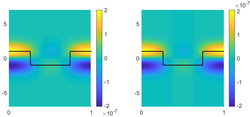
Figure 6: Left: E^\varepsilon(x, y) = n^\varepsilon(x, y) - n^0(y) , where n^\varepsilon(x, y) is determined numerically. Right: theoretical \varepsilon \bar{D}(x, y) . In black, the 1-periodic function \theta given by (152) with a = 0.52 . Here A = 0.9 and \varepsilon = 10^{-4} .
