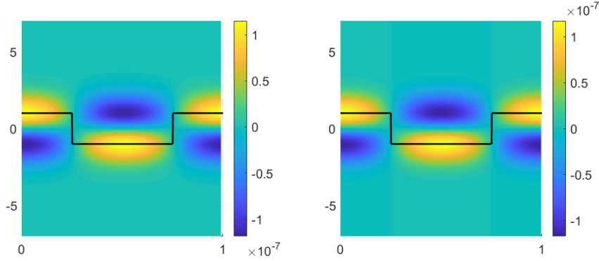
Figure 4: Left: E^\varepsilon(x,y) = n^\varepsilon(x,y) - n^0(y) , where n^\varepsilon(x,y) is determined numerically. Right: theoretical \varepsilon\bar{D}(x,y) . In black, the 1-periodic function \theta given by (152) with a = 0.5 . Here A = 0.9 and \varepsilon = 10^{-4} .
