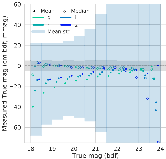
Figure 4. The mean (solid circle) and median (hollow diamond) difference in measured vs. injected magnitude ( \langle\Delta\text{mag}\rangle ) as a function of input magnitude for the final blank image runs with zero-mean Gaussian background noise. The vertical bars correspond to the mean of the standard deviations of griz magnitude responses in each truth magnitude bin, centered at the mean magnitude response. The vertical bars represent the average of the standard deviations of griz magnitude responses in each bin of size 0.5 mag, centered at the mean magnitude response. The overall calibration is excellent, with the median response less than 5 mmag in all bins except for g < 18.5 and 22.5 < z < 23 . We expect significant biases past magnitude 23 due to selection effects near the detection threshold. However, the mean responses show some bias—particularly on the bright end. As discussed in the text, this is due to an asymmetric tendency for SOF to measure the fluxes of bright, extended galaxies to be too large when neighbors are contained in the object’s MEDS stamps. The errors in \langle\Delta\text{mag}\rangle do not substantially decrease past input magnitudes of 20 for the same reason. This is discussed in greater detail in Section 4.3.1.
