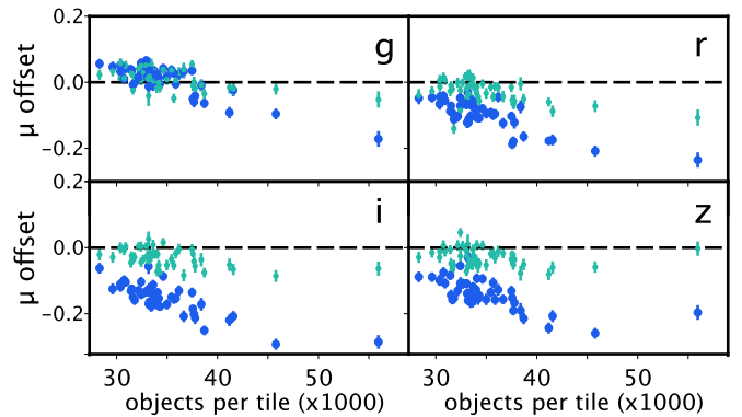
Figure 25. Reproduced from Eckert et al. (2020), Figure 3. The Gaussian mean offset \mu in the BFD flux moment pull distribution as a function of object density for the 48 used Balrog tiles in blue. The green points show the mean offset for the tiles after a local sky subtraction that mitigates the flux bias. While the g band is relatively unaffected, the redder riz bands show statistically significant sky oversubtraction that is correlated with object density.
