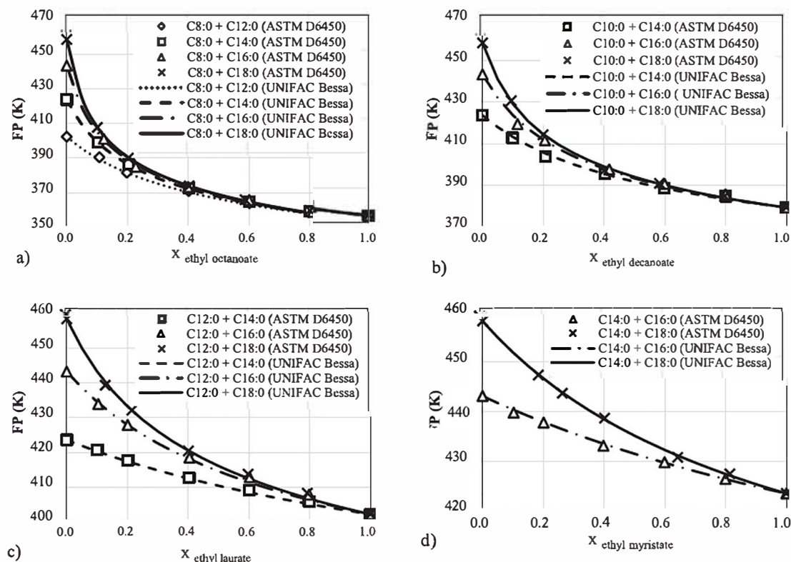
Fig. 2. FP experimental and predicted values (UNIFAC Bessa/Method 2) of Saturated FAEE binary mixtures.
