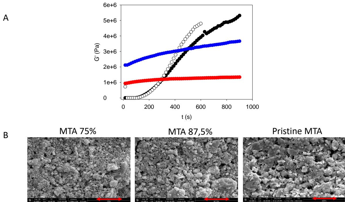
Fig.3: A: Setting kinetics of the pristine MTA ( \circ , \bullet - 2 independent experiments), of the MTA 87.5% ( \bullet ) and of the MTA 75 % ( \bullet ) samples as measured by rheology.
