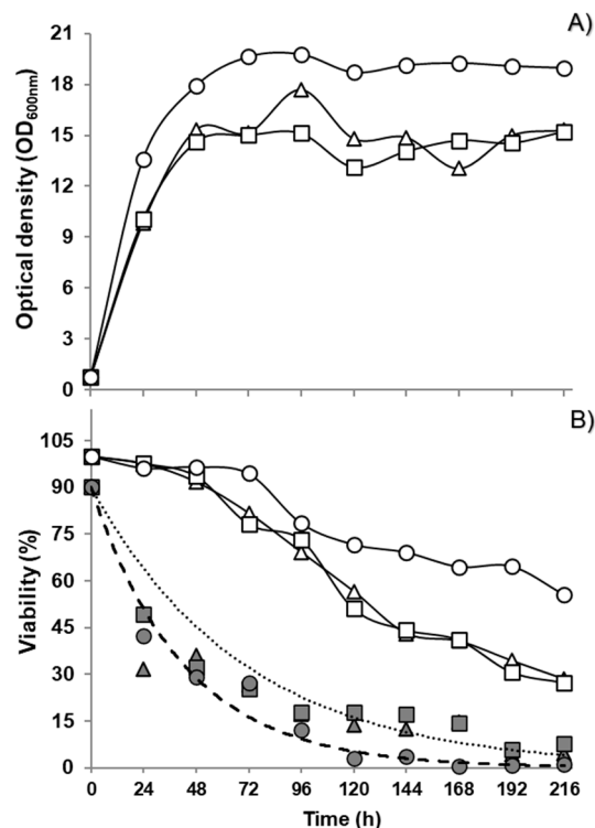
Figure 3. Culture growth on grape juice medium for the three Saccharomyces cerevisiae / Torulasporea delbrueckii mixed inoculum fermentations tested, expressed as: (A) Optical density at 600 nm, (—Δ—) Sc3Y4/Td1AN9, (—□—) Sc3Y8/Td1AN9; (—O—) Fermichamp/Td1AN9; and (B) Percentage of viability of the whole culture (open markers, determined by methylene blue staining) and that of Torulasporea delbrueckii as determined on WL Differential and WL Nutrient agar media, (⋯△⋯) Sc3Y4/Td1AN9, (---■---) Sc3Y8/Td1AN9; (---●---) Fermichamp/Td1AN9. Exponential decay fittings shown with dotted and slashed lines. Standard deviations were always less than 10%; hence, the deviation bars are omitted in the graphs for clarity.
