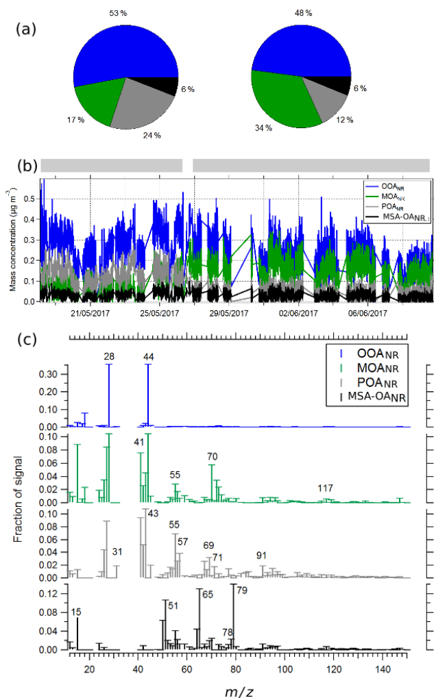
Figure 4. (a) The contribution of the different organic factors during different periods of the PEACETIME ship campaign (identified by the grey bars at the top of b). (b) The mass concentrations of each factor (OOANR, MOANR, POANR, and MSA OANR) as a function of time. (c) The mass spectra of the factors.
