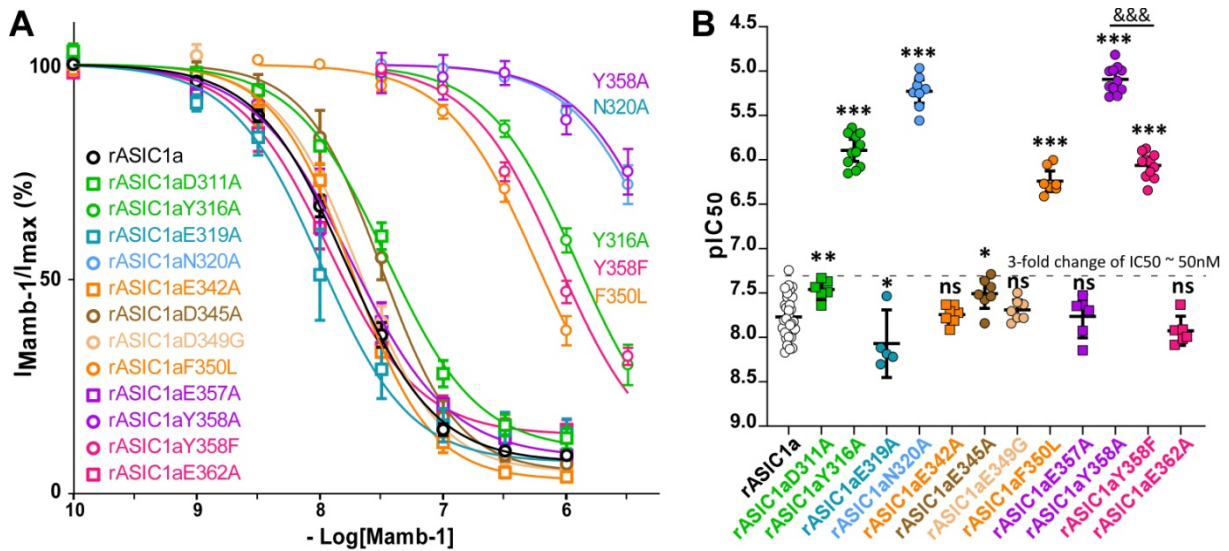
Figure 3. Dose-response curves for inhibition of rASIC1a and its mutants by Mamb-1. A) Fits of the mean values of each data point to a sigmoidal dose-response curve. Mamb-1 was applied for 30 s at pH 7.47 before acid stimulation at pH 5.0. B) Statistical analysis of pIC_{50} calculated from the sigmoidal fits of each recording performed for determination of the mean dose-response curves shown in A ( pIC_{50} as mean with 95% confidence interval, n = 5-31 ; see statistical analysis in Table 2). Significances were calculated with one-way analysis of variance followed by a Dunnett-test (ns P > 0.05 , *P < 0.05 , ***P < 0.001 ; when compared to wild-type rASIC1a noted in white, and t-test between Y358F and Y358A, \&\&\&P < 0.001 ; n = 11 ). The Y316F mutant, which has the same behavior than wild-type rASIC1a (see Figure 2A-B), was not analyzed.
