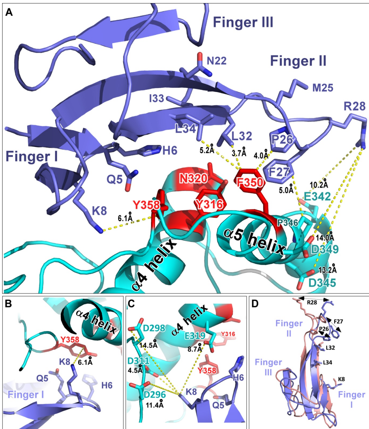
Figure 5. Molecular dynamics simulation of the rASIC1a/Mamb-1 complex. A) View of the interface between fingers I/II of Mamb-1 and \alpha 4/\alpha 5 helices in the thumb domain of rASIC1a. Mamb-1 is shown in dark blue, rASIC1a in cyan blue, and the four key residues forming the hinge in red. Estimated distances between certain residues are indicated by yellow dashed lines. Interactions could occur between the side chains of Lys-8 and Tyr-358, and between the side chains of Leu-32 and Phe-350 as also suggested by double mutant cycle analysis (this study and Mourier et al., 2016). Arg-28 side chain is freely exposed to the solvent and cannot be assigned to neither Glu-342, Asp-345 nor Asp-349 as also suggested by SAR analysis. B) Potential contacts between finger I of Mamb-1 and \alpha 4 helix in the thumb domain of rASIC1a. The estimated distance between Lys-8 and Tyr-358 is indicated. The side chain of Gln-5 does not seem to establish a contact with the side chain of Tyr-358, which is
