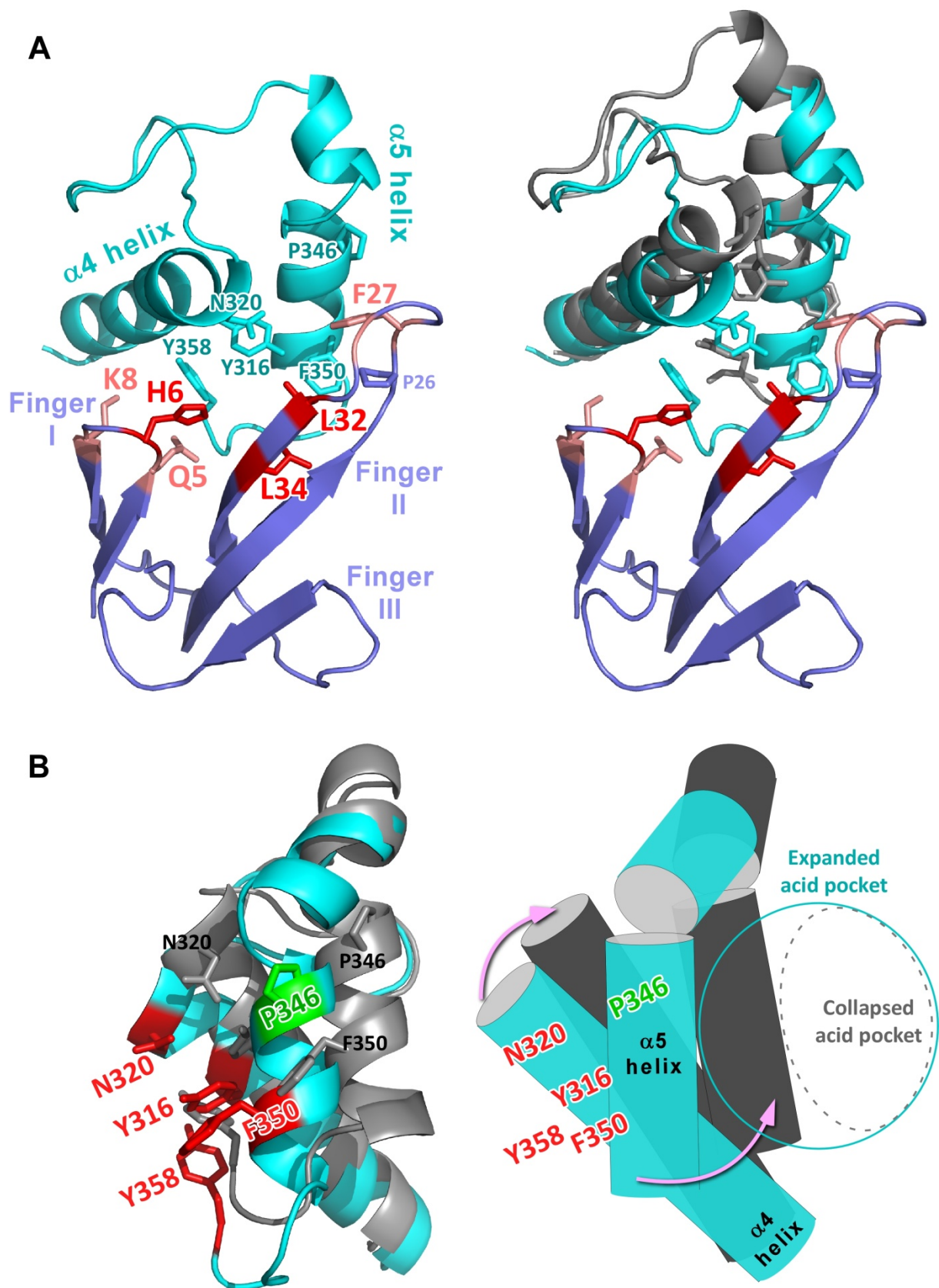
Figure 6. A structural model of rASIC1a inhibition by Mamb-1. A) Fingers I and II of Mamb-1 stabilize the hinge between \alpha 4 and \alpha 5 helices in the thumb domain of the channel (cyan) in a conformation similar to the closed state that is different from the desensitized/open
