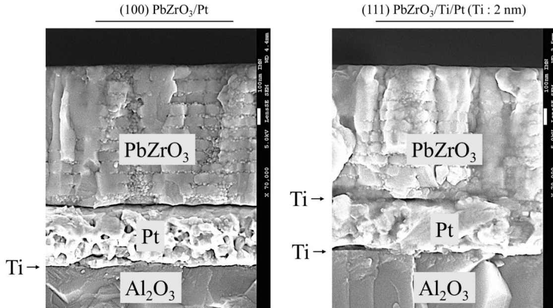
Fig. 4. Cross-sectional SEM morphology of (100) and (111) PbZrO 3
