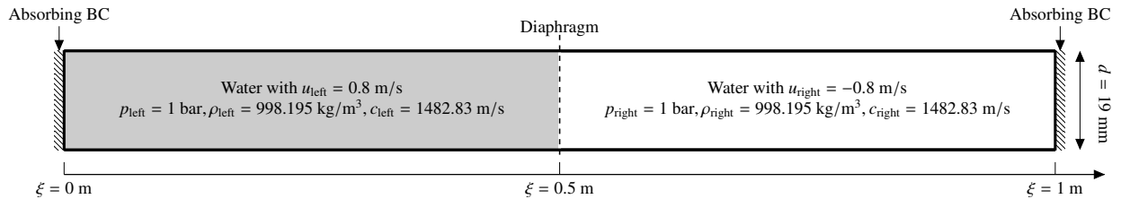
Figure 9: Test description of the double shock-wave problem in liquid water.
