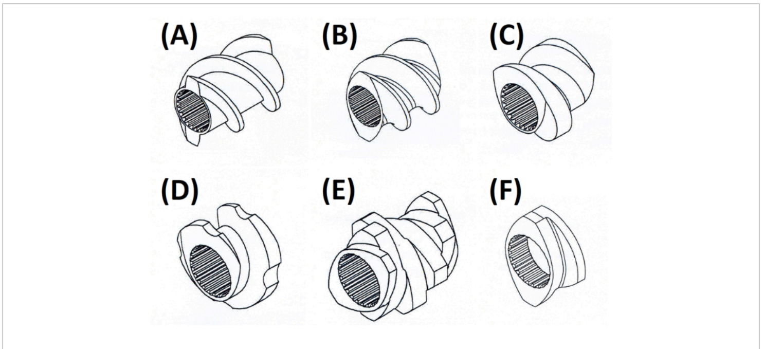
Figure 2: Type of screw elements used along the screw profiles: (A) T2F, (B) C2F, (C) C1F, (D) CF1C, (E) BB, and (F) INO0 screw elements. (A) T2F elements are trapezoidal double-flight screws used for their conveying action. Due to the trapezoidal shape of their threads, T2F elements are non-self-cleaning screws but have very good conveying and swallowing characteristics. They are, therefore, positioned in the feeding areas of the two solids used (i.e., oleaginous flax shives, and plasticized linseed cake). (B) C2F elements are conjugated double-flight screws also used for their conveying action. The shape of their threads is conjugated, which makes the C2F elements self-cleaning screws. They are positioned where the solid and liquid coexist. (C) C1F elements are single-flight screws. In comparison to C2F elements, these conveying screws have a wider thread crest. Therefore, they have a better thrust and a higher shear effect than C2F elements. (D) CF1C elements are conjugated cut-flight, single-flight screws with left-handed pitch. These reverse screw elements are the most restrictive and most important elements of the screw profile. They allow an intense mixing and mechanical shearing of the material as well as an increase of its residence time. CF1C screws are the place where the defibration of the fibers takes place. (E) BB elements are bilobed paddles. They allow a strong mixing effect on the material. They, therefore, promote an intimate mixing action that is particularly important for homogeneously impregnating the oleaginous flax shives with the added water on the one hand, and intimately mixing the extrusion-refined fibers and plasticized linseed cake on the other. (F) INO0 elements are linking elements between double- and single-flight screws. Please click here to view a larger version of this figure.
