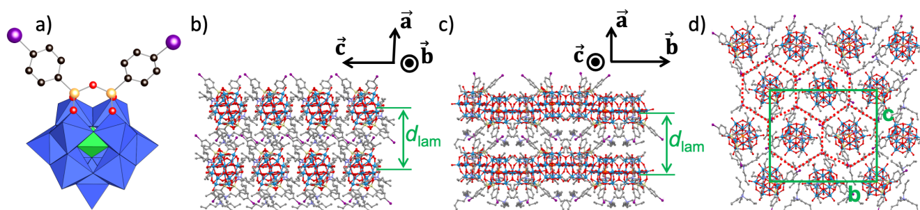
Figure 3. Left: Combined polyhedral/ball-and-stick representation of K Si [I] . Solvent molecules and counterions have been omitted for clarity. WO 6 and PO 4 polyhedra are shown in blue and green, respectively. The Si, O, C and I atoms are shown in orange, red, black and purple respectively; b) rows of aligned POM units directed along b -axis and assembled into layers in the b × c plane; d_{\text{lam}} is the lamellar periodicity; c) side-view of the rows evidencing the alternative up and down orientation of substituents; d) rectangular sublattice (green frame) formed by the honeycomb arrangement of TBA around POM (red dotted lines).
