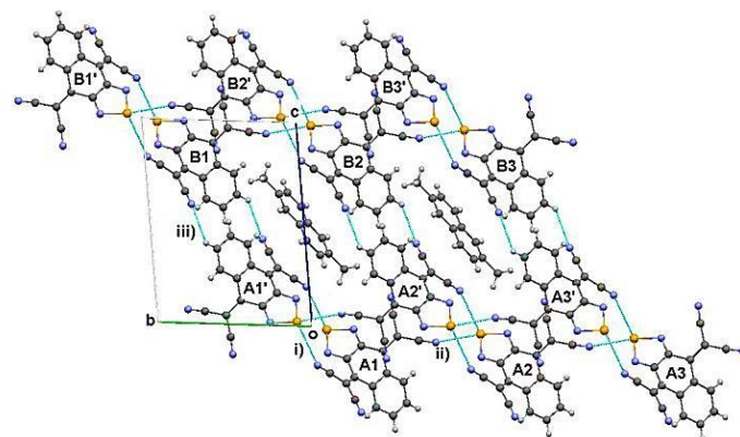
Figure 2. Cavity formation between two dyad-ribbon networks in 2,6-DMN• 1 (1:2) CT crystal. Molecules A1 and A1' forms dyad by ChB through contact (i). Molecules A1, A2, and A3 (as well as A1', A2', and A3') are connected by ChB through contact (ii) to form the dyad-ribbon network. Two dyad-ribbons (A1-A3' and B1-B3') are connected by C-H...N≡C bonds (iii) at different sites (A1' and B1) from those of uncomplexed 1 .
