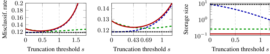
Figure 4: Clustering performance (left, a zoom-in in middle) and storage size (MB) (right) of f_1 (blue), f_2 with M = 2 (green), f_3 (red), and linear f(t) = t (black), versus the truncation threshold s , for SNR \rho = 2 , c = 1/2 and n = 10^3 , with 64 bits per entry for non-quantized matrices.
