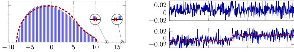
Figure 2: (Left) Histogram of eigenvalues of \mathbf{K} (blue) versus the limiting spectrum and spikes (red). (Right) Eigenvectors of the largest (top) and second largest (bottom) eigenvalues of \mathbf{K} (blue), versus the rescaled class label \alpha \mathbf{v} / \sqrt{n} (red, from Corollary 2). f(t) = \sin(t) - 3 \cos(t) + 3/\sqrt{e} , p = 800 , n = 6400 , \mu = 1.1 \cdot \mathbf{1}_p / \sqrt{p} , \mathbf{v} = [-\mathbf{1}_{n/2}; \mathbf{1}_{n/2}] on Student-t data with \kappa = 5 .
