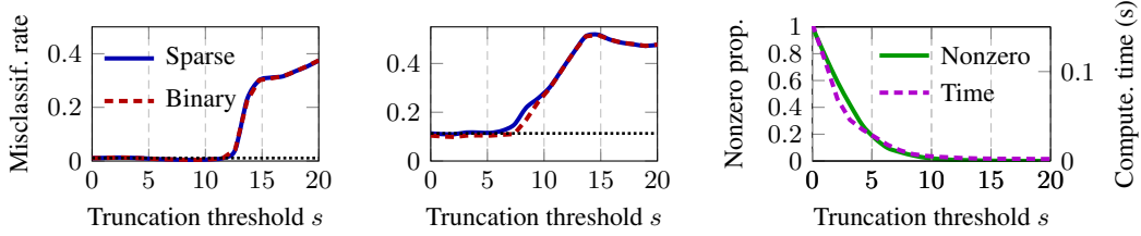
Figure 7: Clustering performance of sparse f_1 and binary f_3 (left and middle), proportion of nonzero entries and computational time of the top eigenvector for f_3 (right), as a function of the truncation threshold s on the MNIST dataset: digits (0, 1) (left) and (5, 6) (middle and right) with n = 2048 and performance of the linear function in black. Results averaged over 100 runs.
