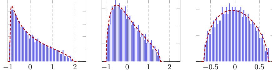
Figure 11: Eigenvalues of \mathbf{K} with \mu = 0 (blue) versus the limiting laws in Theorem 1 and Corollary 3 (red) for Gaussian data, p = 1024 , n = 512 and f(t) = t \cdot 1_{|t| > \sqrt{2}s} with s = 0.1 (left), s = .75 (middle), and s = 1.5 (right).
