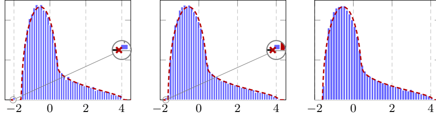
Figure 12: Eigenvalues of \mathbf{K} with \mu = 0 (blue) versus the limiting laws and spikes in Theorem 1 and Corollary 1 (red) for Student-t (with 7 degrees of freedom, left), Gaussian (middle) and Rademacher distribution (right), p = 512 , n = 2048 , f(t) = \max(t, 0) - 1/\sqrt{2\pi} . Emphasis on the non-informative spikes at different locations: at -2.10 for Student-t and -1.77 for Gaussian.
