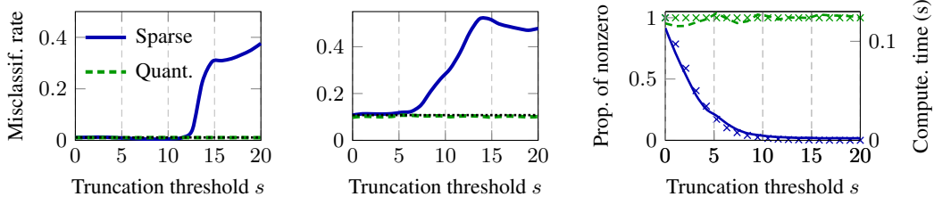
Figure 14: Clustering performance ( left ), proportion of nonzero entries, and computational time of the top eigenvector ( right , in markers) of sparse f_1 and quantized f_2 with M = 2 , as a function of the truncation threshold s on the MNIST dataset: digits (0, 1) ( left ) and (5, 6) ( middle and right ) with n = 2048 and performance of the linear function in black . Results averaged over 100 runs.
