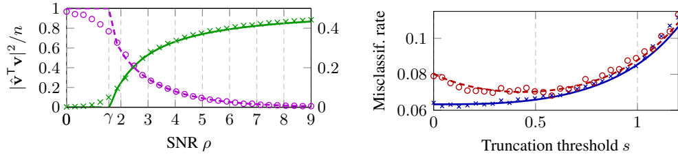
Figure 3: (Left) Empirical alignment |\hat{\mathbf{v}}^T \mathbf{v}|^2/n ( green crosses ) and misclassification rate ( purple circles ) in markers versus their limiting behaviors in lines, for f(t) = \text{sign}(t) , as a function of SNR \rho . (Right) Misclassification rate as a function of the truncation thresholds s of sparse f_1 ( blue crosses ) and binary f_3 ( red circles ) with \rho = 4 . Here, p = 512 , n = 256 , \boldsymbol{\mu} \propto \mathcal{N}(\mathbf{0}, \mathbf{I}_p) , \mathbf{v} = [-\mathbf{1}_{n/2}; \mathbf{1}_{n/2}] on Gaussian data. The results are obtained by averaging over 250 runs.
