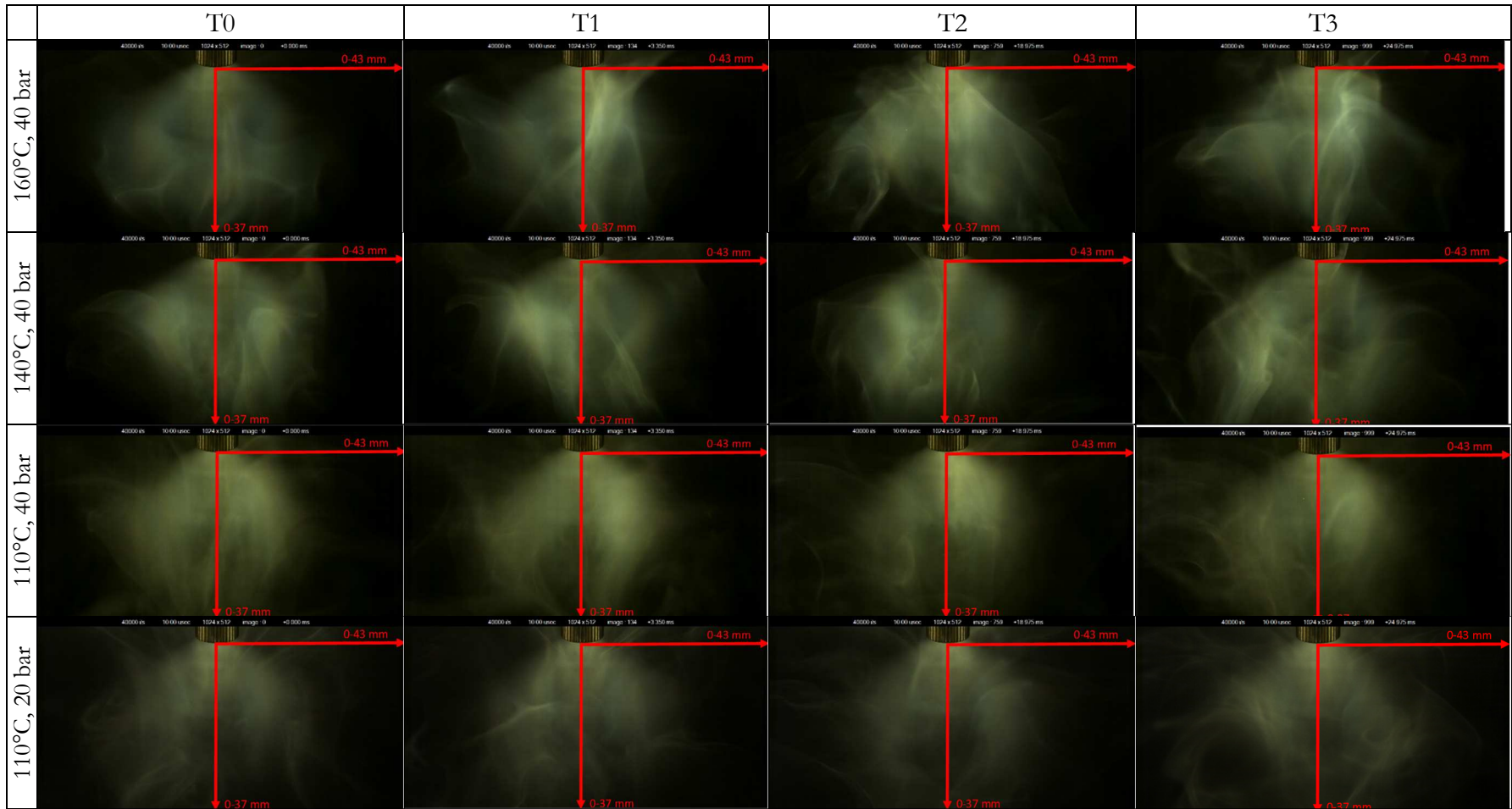
Fig. 7. Acetone spray under different operating conditions at T0, T1 (3350ms), T2 (18975ms) et T3 (74975ms)
