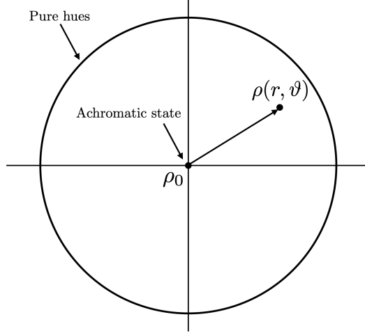
Figure 4: The unit (Bloch) disk \mathbf{D} in \mathbb{R}^2 , whose points represent quantum chromatic states. The points of its border S^1 represent pure quantum chromatic states and the center represents the achromatic state.
