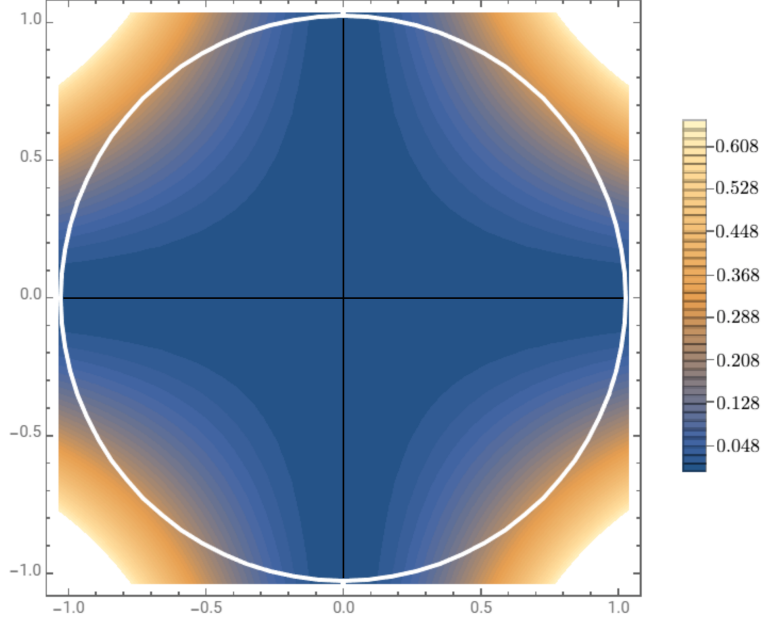
Figure 5: The polar graph of the lower bound \frac{r^4}{4} \sin^2(2\vartheta) of eq. (60). Notice that this lower bound is 0 only for points with coordinates (r, \vartheta) lying on the opponency axes, identified with the horizontal and vertical axes in the picture. The lower bound is maximal for (r, \vartheta) = (1, \frac{\pi}{4} + k\frac{\pi}{2}) , k = 1, 2, 3 .
