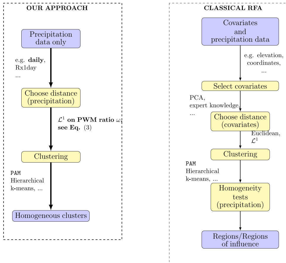
Fig. 2. Steps to delineate homogeneous regions in RFA (traditional vs. method introduced in this paper). Rx1day is the annual maximum daily precipitation. The left method corresponds to the methods developed in this paper. The other way is the traditional RFA path with homogeneity tests, see e.g. Hosking and Wallis (2005).
