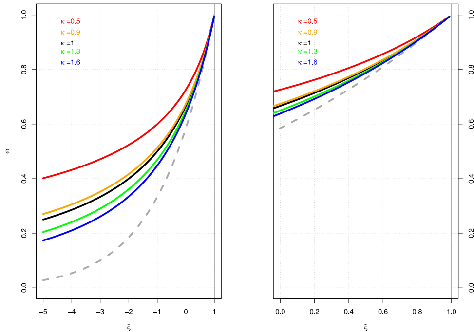
Fig. 3. The y-axis represents the ratio \omega for a EGPD( \kappa, \sigma, \xi ), see Eq. (4). The x-axis corresponds to the upper tail shape parameter \xi . The left panel has \xi \in (-5, 1) while the right panel provides a zoom on \xi \in (0, 1) . Each color represents a different value of \kappa \in \{.5, .9, 1, 1.3, 1.6\} . The gray dotted line corresponds to the GEV case. The black line with \kappa = 1 corresponds to the GP case. (For interpretation of the references to color in this figure legend, the reader is referred to the web version of this article.)
