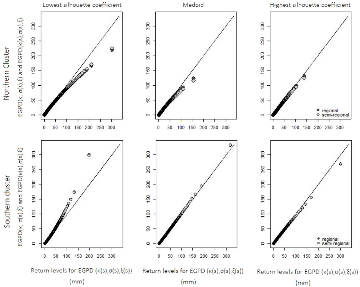
Fig. 9. Comparison of quantile–quantile plots: The x-axis corresponds to the local quantiles from Model (7). The y-axis displays semi-regional and regional quantiles, i.e. from models (9) and (8), respectively. Rows indicate the cluster family, alpine or low altitude area, and the column corresponds to the station type: the worst (best) classified station in the first (third) column. The medoid station is represented by the middle column.
