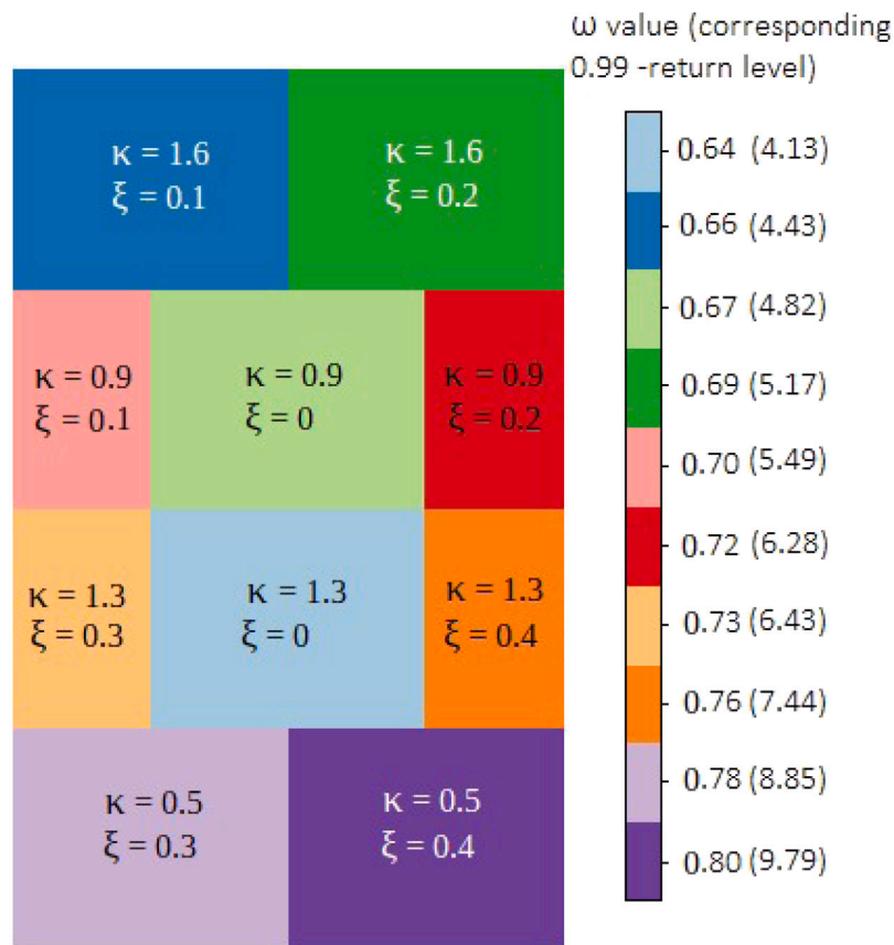
Fig. 4. Experimental design setup based on EGPD( \kappa, \sigma, \xi ), see Eq. (4). The colors correspond to 10 values of the ratio \omega with their associated \kappa and \xi parameter values. A large (small) rectangle contains 40 (20) locations. The numbers in brackets in the color legend represent the 99% return level associated with each combination. (For interpretation of the references to color in this figure legend, the reader is referred to the web version of this article.)
