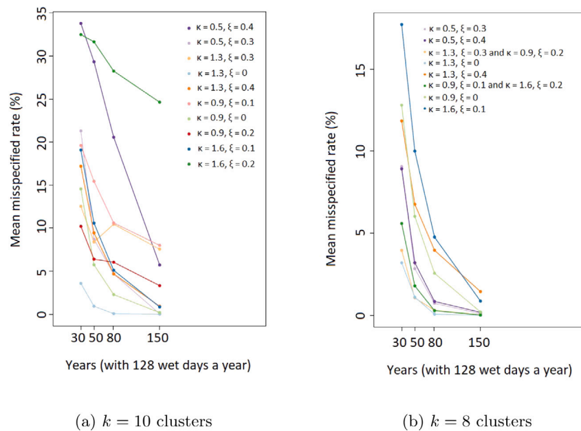
Fig. 5. Misspecified PAM clustering rates with respect to the 10 regions shown in Fig. 3 for k chosen as input in PAM algorithm. k = 10 (Panel (a)) corresponds to the number of simulated homogeneous regions. The case k = 8 (Panel (b)) corresponds to an underestimation of the number of homogeneous regions (e.g. for small samples).
