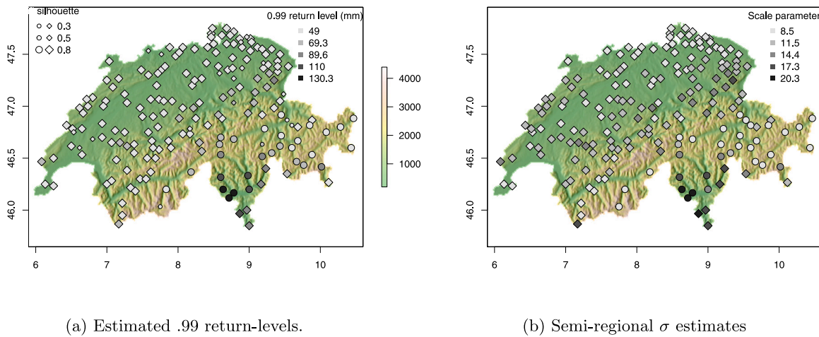
Fig. 7. Swiss daily precipitation modeled with the regional Model (8): Panel (a): PAM outputs in two clusters that are identified by circles (so-called “low altitude area cluster”) and diamonds (so-called “alpine cluster”), see also Fig. 10. The size of the points is proportional to the silhouette coefficient. The gray nuance color legend corresponds to .99 return level fits from Model (8). Panel (b): Estimates of \sigma in Model (8).
