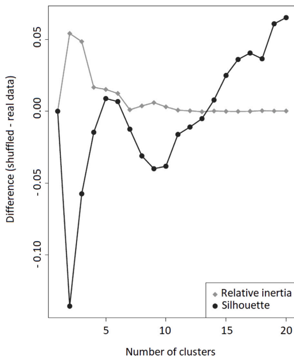
Fig. 6. Swiss daily precipitation. Differences of relative inertia and silhouette coefficient between shuffled data and observed daily precipitation as a function of the number of clusters.
