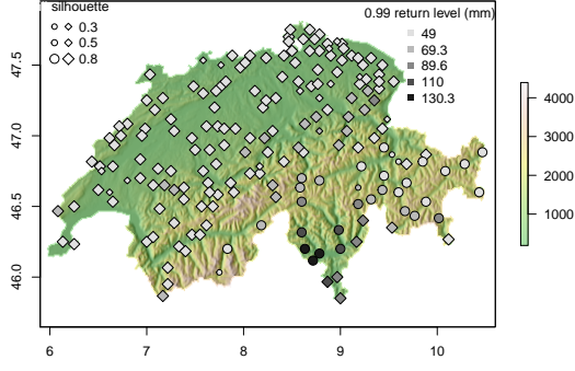
(a) Estimated .99 return-levels.
