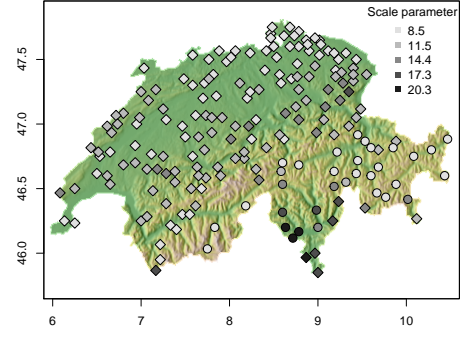
(b) Semi-regional \sigma estimates
