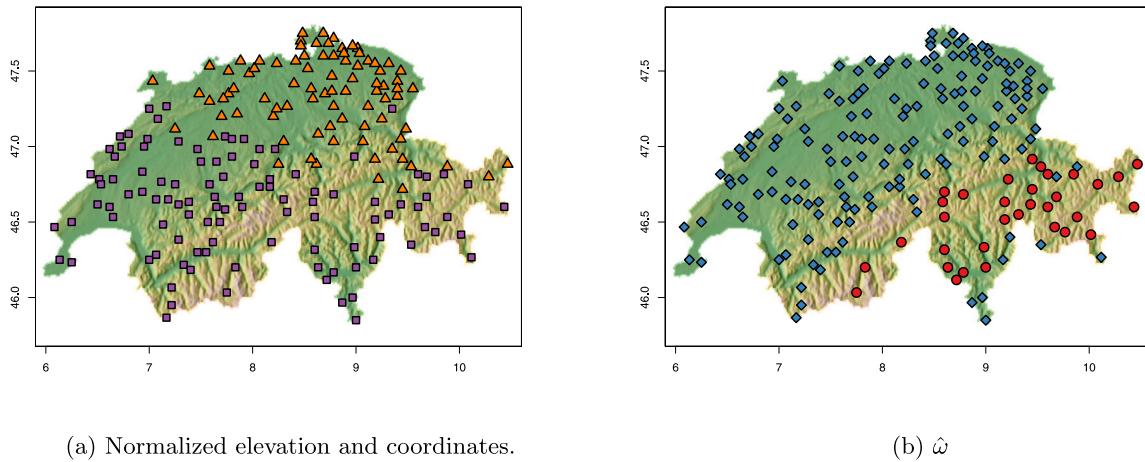
Fig. 10. Partition of Swiss weather stations applying PAM algorithm to covariates (traditional RFA approach, see Hosking and Wallis, 2005) or \hat{\omega} (our method). Shape and color of the points indicate their cluster. (For interpretation of the references to color in this figure legend, the reader is referred to the web version of this article.)
