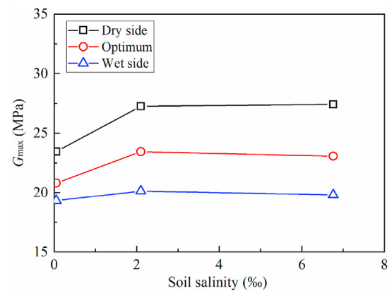
Fig. 6. Salinity effect on small-strain shear modulus.
