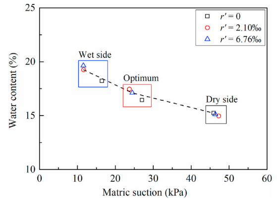
Fig. 5. Matric suction of compacted samples on dry and wet sides and at optimum state.
