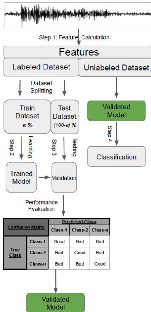
Figure 4: Workflow of the machine learning process. Step 1: Feature calculation step to represent the signals. Step 2: Learning step on a given proportion of the dataset. Step 3: Testing step to evaluate the performance of the model. Step 4: Classification step on new, unlabeled data with a validated model, as the operational part of the process.
