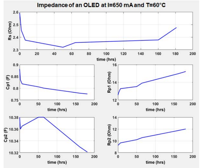
Fig. 8. Impedance evolution of a tested OLED at I = 650 \text{ mA} and T = 60^\circ C
