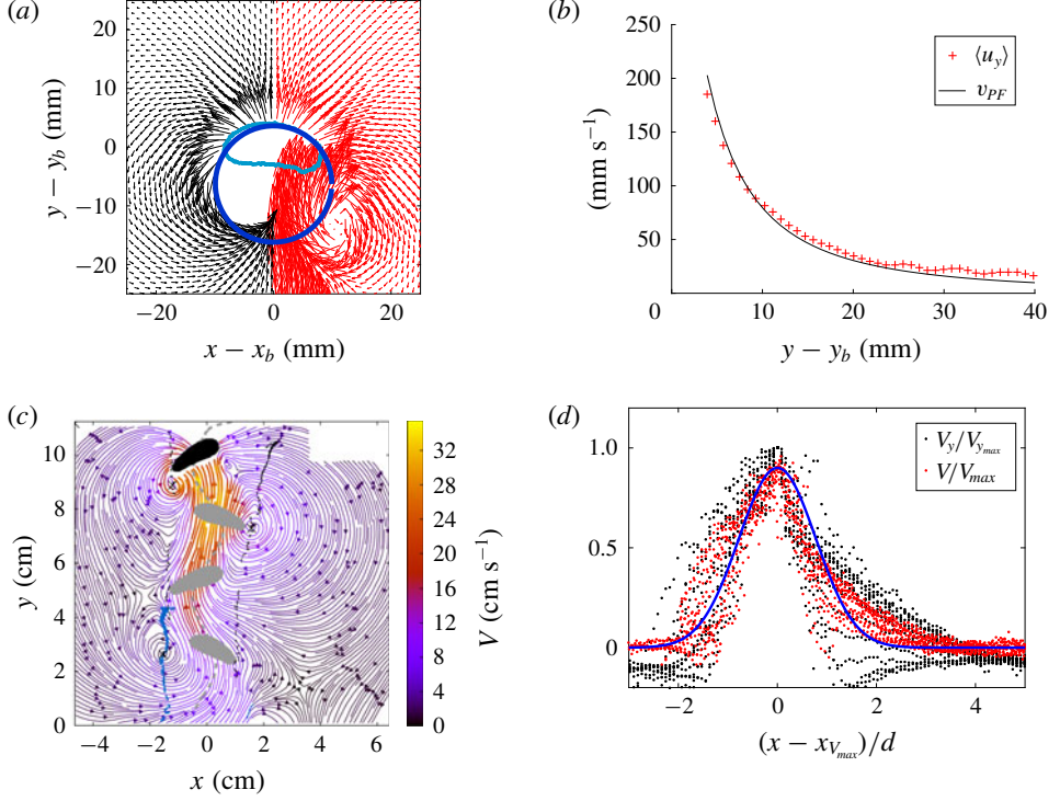
FIGURE 2. Illustration of the liquid velocity around a single bubble at Ar = 4380 . (a) Potential flow in front of the bubble; comparison between the velocity field measured by PIV around a single bubble (red arrows) with the potential flow around the blue circle of radius r = d\sqrt{\chi}/2 centred in y - y_b = d/(2\sqrt{\chi}) - r (black arrows). (b) Comparison between the vertical velocity profiles along the vertical direction measured by PIV and predicted by potential flow at x = x_b . (c) Streamlines in the wake behind a single bubble obtained by PIV measurements; the dashed grey line corresponds to the path of the bubble. The crosses correspond to the centres of the vortices present in the velocity field at the time of measurement. The black (respectively, blue) line indicates the path of a vortex released in (respectively, just before the bubble entered) the measurement window. Thick lines show the paths of the two vortices remaining after vortex pairing. (d) Transverse profiles of the normalized longitudinal velocity in the wake of the bubble; dots: PIV measurements of either the vertical component V_y or of the norm V (normalized with their maximum values); blue line: Gaussian profile \hat{U}_{f1\infty}/V_{max} from (2.3) and (2.4).
