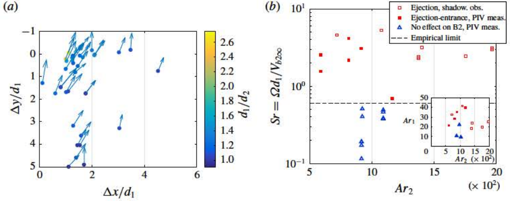
FIGURE 9. Conditions for rapid ejection or centring of B2 in the wake due to the vortices of B1. (a) Positions and normalized velocities of B2 provided by the shadowgraphy observations (velocities are normalized by \sqrt{gd_2} ), (b) limit between observations of ejections or centring of B2 in the wake and observations of no effect on B2 in (Ar_2, Sr) diagram. The insert provides the values of Ar_1 and Ar_2 in the cases for which Sr was directly measured by PIV or estimated from the shadowgraphy observations.
