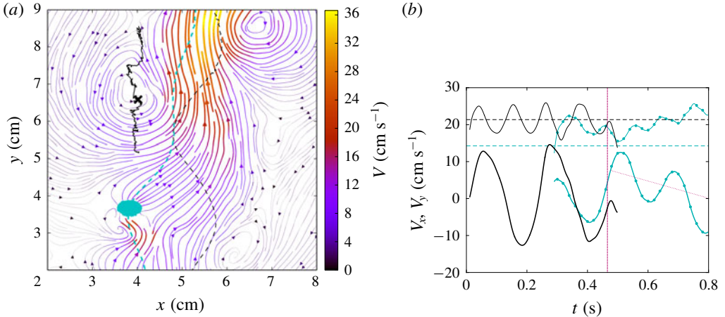
FIGURE 8. Re-alignment or centring of the trailing bubble in the wake of the leading one for Ar_1 = 3900, Ar_2 = 1160 . Same legend as figure 7, the vertical purple dashed line indicating here the time of recentring, t_{rec} . The oblique purple dotted line shows the mean horizontal drift experienced by B2.
