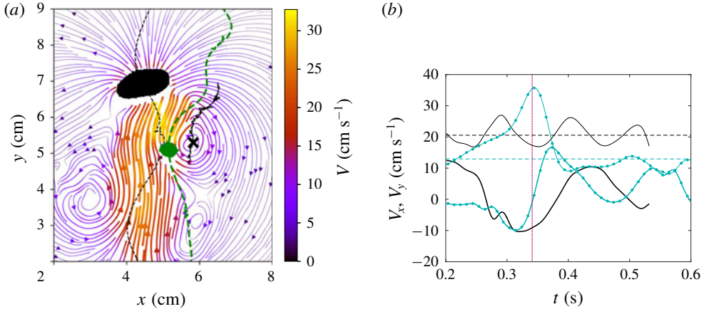
FIGURE 7. Ejection of the trailing bubble for Ar_1 = 3510 , Ar_2 = 880 . (a) Streamlines of the velocity field at the time of ejection t_{ej} with the contours of the bubbles. The black (respectively, green) dashed line corresponds to the path of the leading (respectively, trailing) bubble. The black line corresponds to the path of the vortex which interacts with the trailing bubble. The black cross indicates the centre of this vortex at the time t_{ej} . (b) Velocity components of the bubbles (in black for bubble B1 and in turquoise for bubble B2). Thick (respectively, thin) lines indicates the horizontal (respectively, vertical) velocity. The vertical purple dashed line indicates the time of ejection t_{ej} . The horizontal dashed lines correspond to the terminal velocity of the equivalent isolated bubbles.
