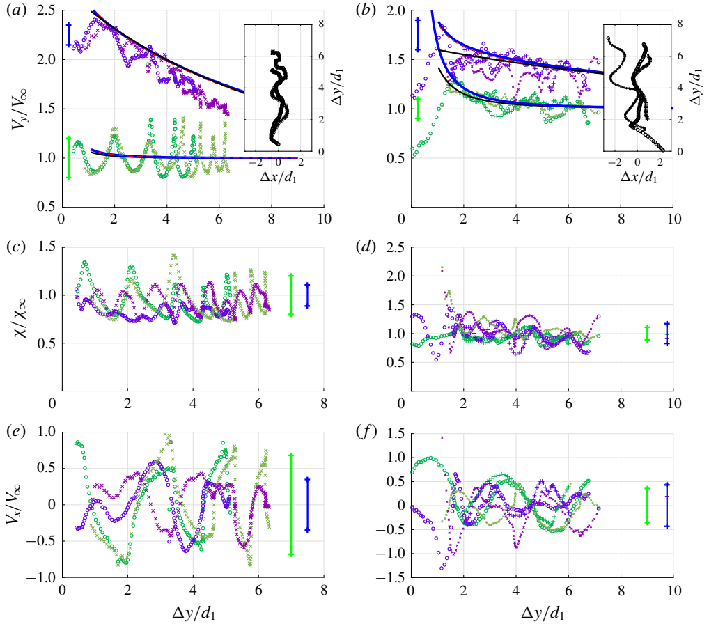
FIGURE 6. Comparison between experiments and the prediction of the entrainment model. Upper figures (a,b): vertical velocity as a function of the separation distance between the two bubbles; Central figures (c,d): elongation ratio; Lower figures (e,f): horizontal velocities. The symbols correspond to two experiments for Ar_1 \approx 4000, Ar_2 \approx 1500 on the left-hand side (crosses report the same case as in figure 3 with Ar_1 = 3820, Ar_2 = 1525 ) in (a,c,e); and to three experiments for Ar_1 \approx 1500, Ar_2 \approx 2000 on the right-hand side in (b,d,f). Purple (respectively, green) symbols correspond to the leading (respectively, trailing) bubble. Purple (respectively, green) vertical bars are representative of the amplitude of the oscillations for isolated bubbles with diameters close to the leading (respectively, trailing) bubble. The solid lines correspond to the predictions of the model (relations (3.4) and (3.5)) with continuous blue line: model with all terms; red dashed line: model without inertial terms (initial conditions are given at \Delta y/d_1 = 10 where both bubbles have their terminal velocity). The black continuous line corresponds to the fluid velocity generated by the other bubble ( 1 + U_{fi}/V_{bj\infty} with i \neq j ). The insert in the upper figures (a and b) shows the relative positions of the bubbles during the interaction.
