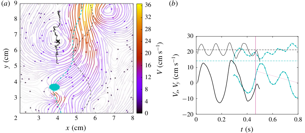
FIGURE 8. Re-alignment or centring of the trailing bubble in the wake of the leading one for Ar_1 = 3900, Ar_2 = 1160 . Same legend as figure 7, the vertical purple dashed line indicating here the time of recentring, t_{rec} . The oblique purple dotted line shows the mean horizontal drift experienced by B2.
