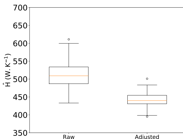
Figure 12: Box plot of the HTC and the adjusted HTC estimates for the increased airtightness configuration
