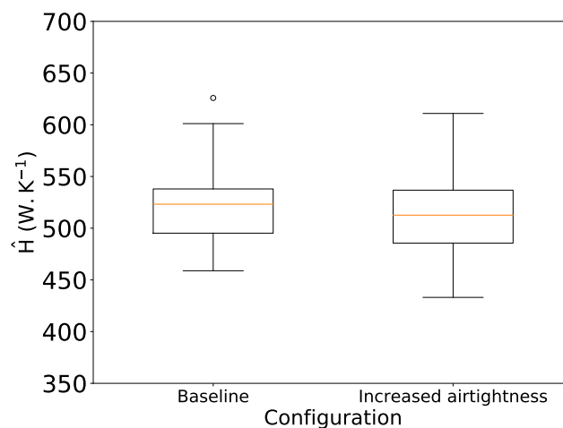
Figure 10: Box plot of the HTC estimates for the baseline and the increased airtightness configurations
