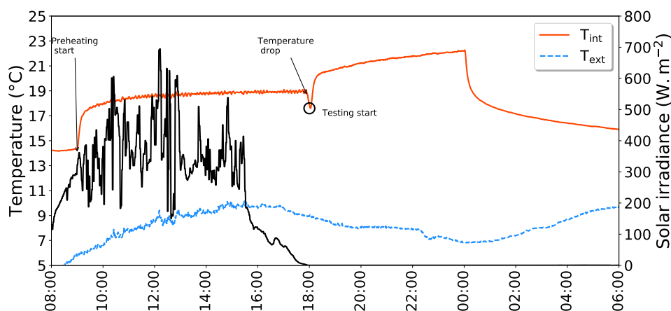
Figure 11: Internal temperature evolution prior to and during a QUB test
