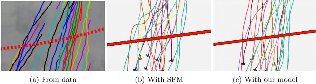
Figure 4: Pedestrians trajectories after a lateral interaction with a car (large red line).
