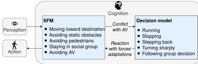
Figure 1: The hybrid model of pedestrians behavior.
