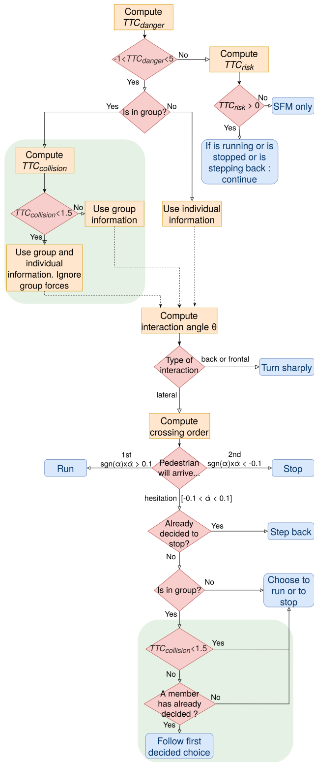
Figure 3: Flowchart of the proposed decision model, with calculations in orange, tests leading to decisions in red and action decided in blue. The two green areas are for groups.
