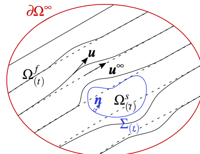
Figure 1. Scheme of the fluid and solid domain.
