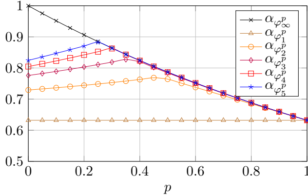
Figure 1: Tight approximation ratios \alpha_{\varphi_{\ell}^p} , where \ell is the rank of the capped version of the p -VEHICLE-TARGET ASSIGNMENT problem. When p = 0 , we recover the \ell -coverage problem.
