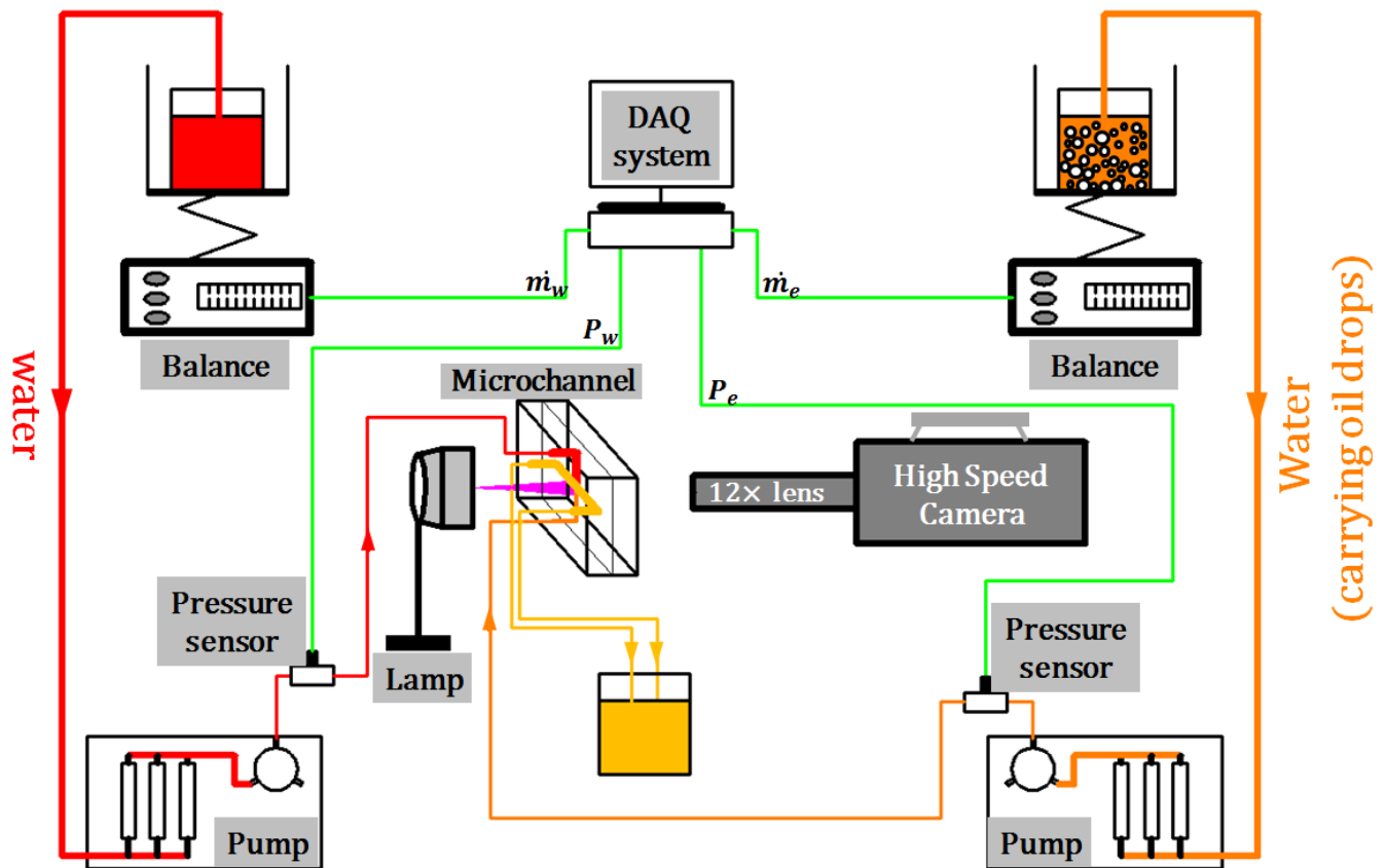
Fig.1 Experimental system for drop breakup observation.
