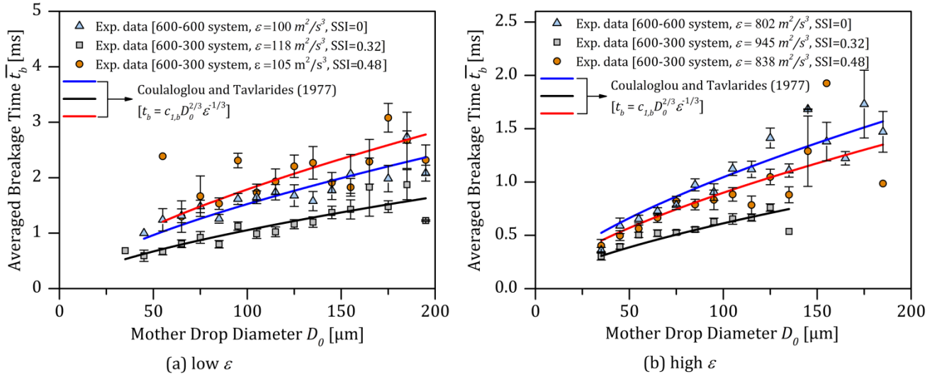
Fig.10 Modeling of averaged breakage time. a) low \varepsilon case: c_{1,b} = 0.073 for 600-600 system; c_{1,b} = 0.052 for 600-300 system, SSI=0.32; c_{1,b} = 0.085 for 600-300 system, SSI=0.48. b) high \varepsilon case: c_{1,b} = 0.050 for 600-600 system; c_{1,b} = 0.029 for 600-300 system, SSI=0.32; c_{1,b} = 0.043 for 600-300 system, SSI=0.48.
