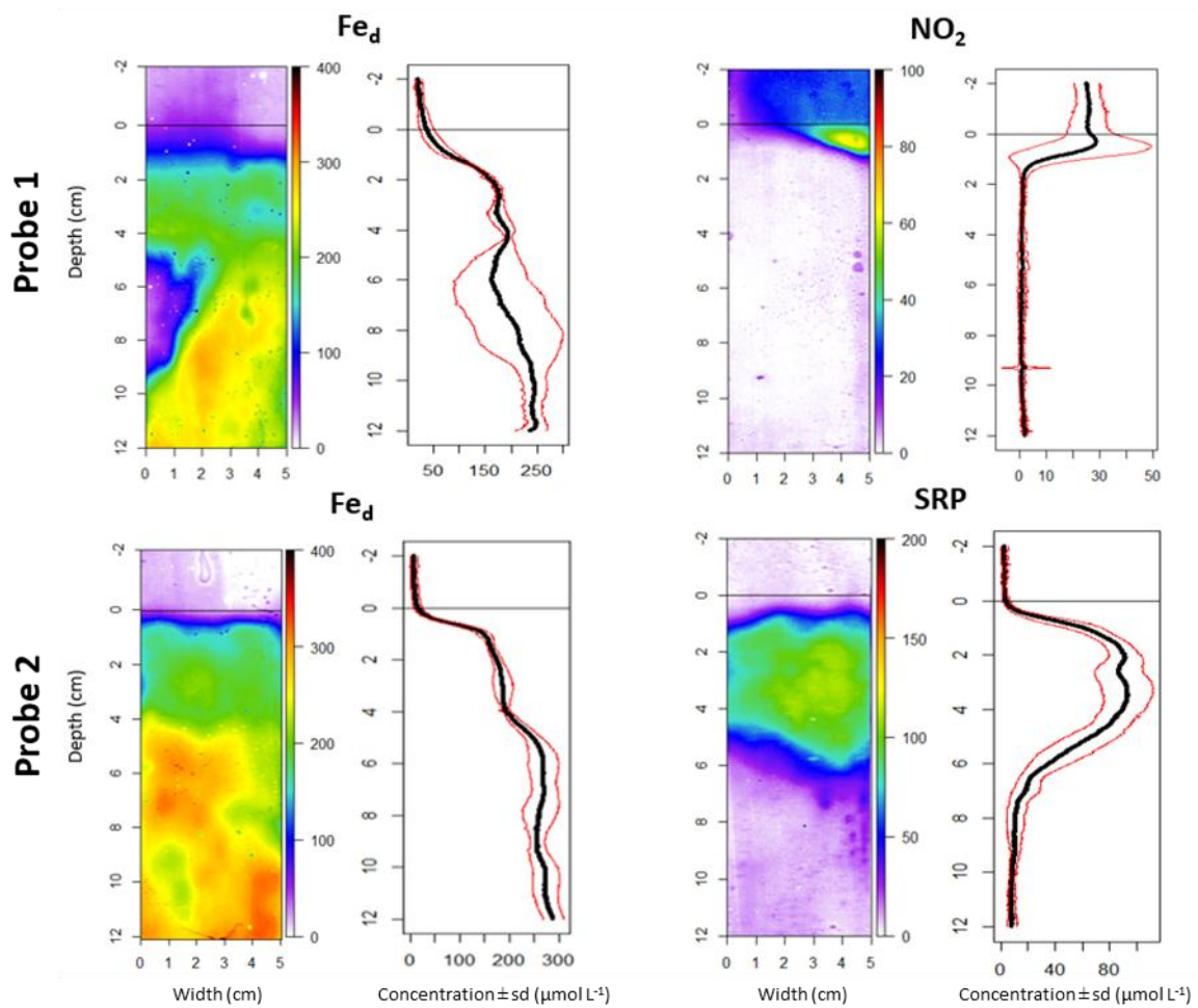
Fig. 4. 2D pore water distribution of iron ( Fe_d ) (probe 1 and 2), nitrite ( NO_2 ) (probe 1) and soluble reactive phosphorus (SRP) (probe 2) concentrations of cores at Marans in April, and their associated 1D profile (black bold line represented the mean concentration, red lines, standard deviation). The horizontal black line represented the SWI. The color scale on the right of each image represented the concentrations in \mu\text{mol L}^{-1} . The probes came from two different cores.
