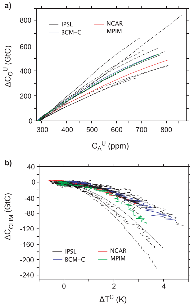
FIG. 1. (a) The global change in cumulated (1860–2100) oceanic \text{CO}_2 uptake (PgC) \Delta C_O^U vs the global-mean annual-mean atmospheric p \text{CO}_2 (ppm) \Delta C_A^U from the “uncoupled” C^4\text{M} simulations of Friedlingstein et al. (2006)—see Eq. (6). The gradient of the relationship represents the global sensitivity of oceanic \text{CO}_2 uptake to rising atmospheric \text{CO}_2 concentrations \beta^U ( \text{PgC ppm}^{-1} ). (b) The global change in climate-induced cumulated (1860–2100) oceanic \text{CO}_2 uptake (PgC) \Delta C_{\text{CLIM}} vs the global-mean annual-mean change in surface atmospheric temperature (K) \Delta T^C from the “coupled” C^4\text{M} simulations of Friedlingstein et al. (2006)—see Eq. (8). The gradient of the relationship represents the global sensitivity of the \text{CO}_2 uptake to climate change \gamma ( \text{PgC K}^{-1} ). In both panels, the models used in this study are highlighted in color and include an additional model, BCM-C, not included in the original study of Friedlingstein et al. (2006).
