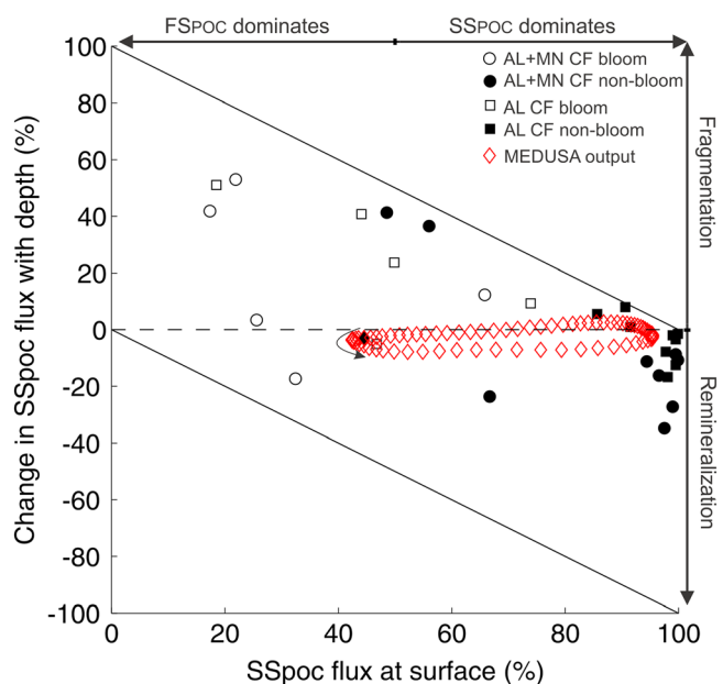
Figure 3. Percentage change in slow-sinking SETCOL POC flux with depth ( SS_{POC} \text{ flux (MLD + 110 m)} \% - SS_{POC} \text{ flux (MLD + 10 m)} \% ) versus the SETCOL SS_{POC} \text{ flux (MLD + 10 m)} at the surface in the Southern Ocean. The circles represent the SS_{POC} percentage fluxes when the Allredge [1998] conversion factors are used for aggregates and the Manno et al. [2015] conversion factor is used for fecal pellets (AL + MN CF). The squares represent the SS_{POC} percentage fluxes when the Allredge [1998] conversion factors are used for aggregates and fecal pellets (AL CF). This allows a comparison between the relative contributions and highlights that, while there is a change in magnitude, the trends are unchanged. The red diamonds indicate the mean annual cycle in the MEDUSA model with the black diamond representing the first time step which continues anticlockwise as shown by the arrow [Yool et al., 2013]. The open symbols represent samples collected during the spring bloom in December 2013, and filled symbols represent samples collected in declining/postbloom phases in January 2013. The black diagonal lines indicate the limits of where it is mathematically possible for the SS_{POC} flux (%) to increase/decrease due to percentages being bounded by 0 and 100. Data points that plot on the zero (dashed) line show no change in the FS: SS_{POC} ratio indicating both fluxes are degraded at the same rate. Data points below the dashed line indicate that SS_{POC} flux decreases in magnitude more rapidly than FS_{POC} flux. Data above the zero line indicate that SS_{POC} flux makes a greater contribution to total POC flux with depth.
