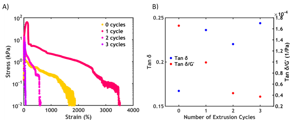
Figure 7 A) Underwater adhesion performance after application of a temperature-salt switch at a nominal strain rate of 0.2 \text{ s}^{-1} . B) \text{Tan } \delta and \text{Tan } \delta/G' recorded with a rheometer at \omega = 1 \text{ rad/s} (comparable to the strain rate in the tack measurement).
