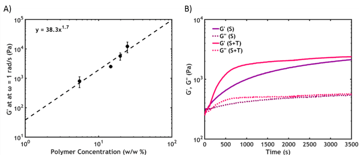
Figure 5 Setting processes. A) Storage modulus recorded at \omega = 1 rad/s after a single temperature switch plotted against the polymer concentration. B) Time sweeps after one extrusion cycle when performing a salt (S) or a combined salt and temperature (S+T) switch;
