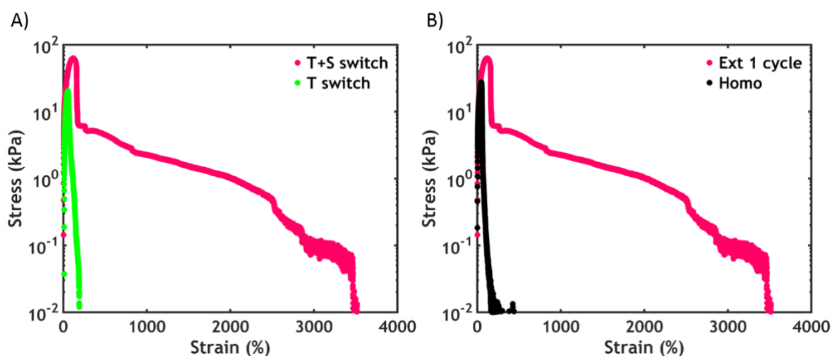
Figure 8 Underwater adhesive performance of the sample extruded once after application of a temperature-salt switch compared to A) the application of a single temperature switch and B) the performance of the homopolymer complex coacervate upon a combined trigger.
