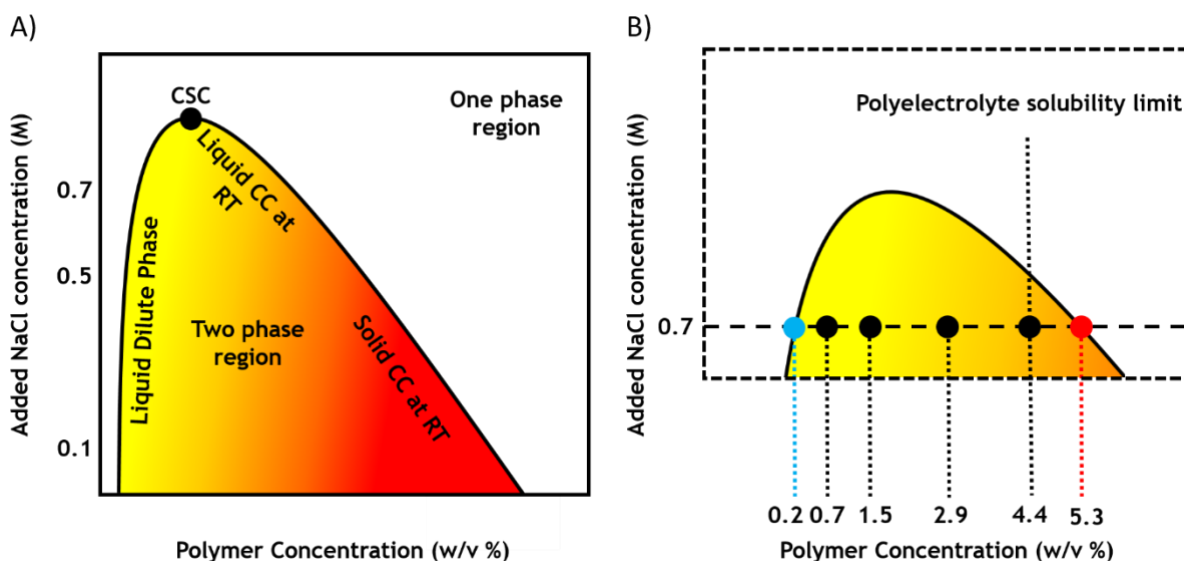
Figure 2 A) Complex coacervate (CC) phase diagram. In the two phase region a gradient from yellow to red is used to indicate the transition from a liquid dilute phase (left side) to a liquid CC phase (top right side) and finally to a solid CC phase (bottom right side). B) Effect of polymer concentration: zoom in the liquid CC area, in which the black dots represent the analysed samples, which phase separate into a dilute phase, shown as a light blue dot, and a complex coacervate phase, shown as a red dot.
