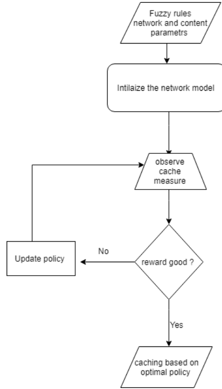
Figure 4: block diagrame of caching over mRL
