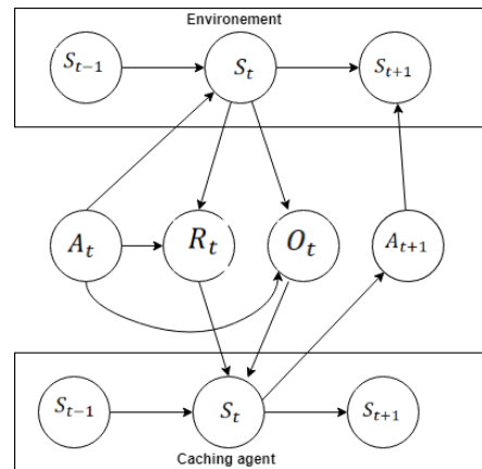
Figure 5: cahing Agent process
