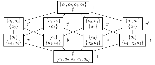
Figure 2: The formal concept lattice of R .
