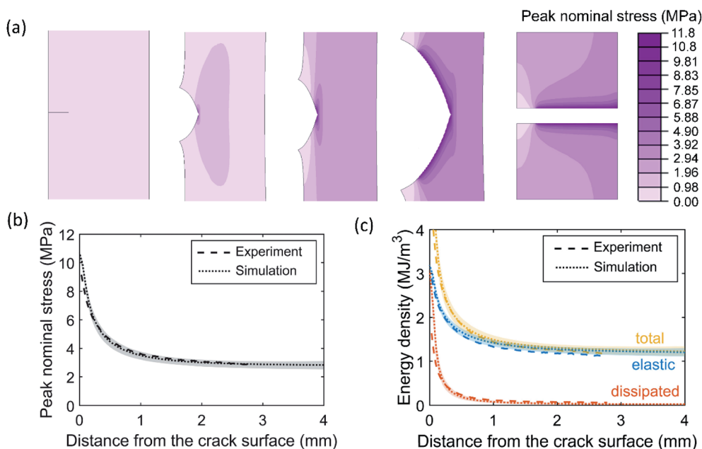
Fig. 5 FE simulation of crack propagation in the EA0.2-0.05(2.61) SEN sample. (a) Contour of peak nominal stress before, during and after crack propagation. (b) and (c) Comparison between simulation results and experimental data in terms of (b) the peak nominal stress and (c) the total, elastic and dissipated energy densities in the completely fractured SEN sample. The shaded regions represent ranges of the simulation results and the dotted lines represent the averages of simulation results.
