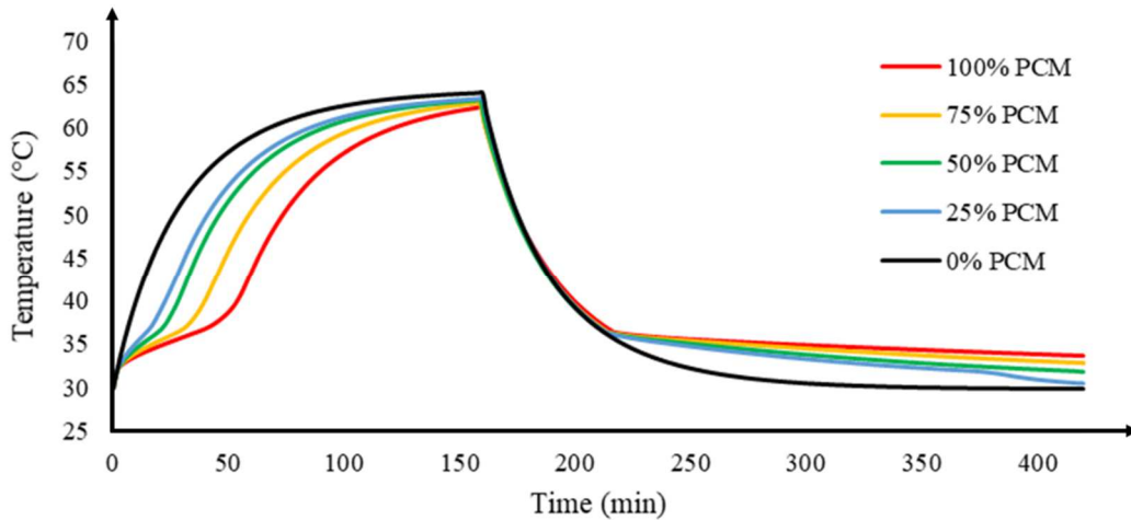
Figure 11. Variation of the temperature profile for different volume fraction of PCM
