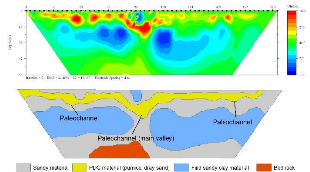
Figure 5. Suspected paleo-channel generated from resistivity data interpretation.
