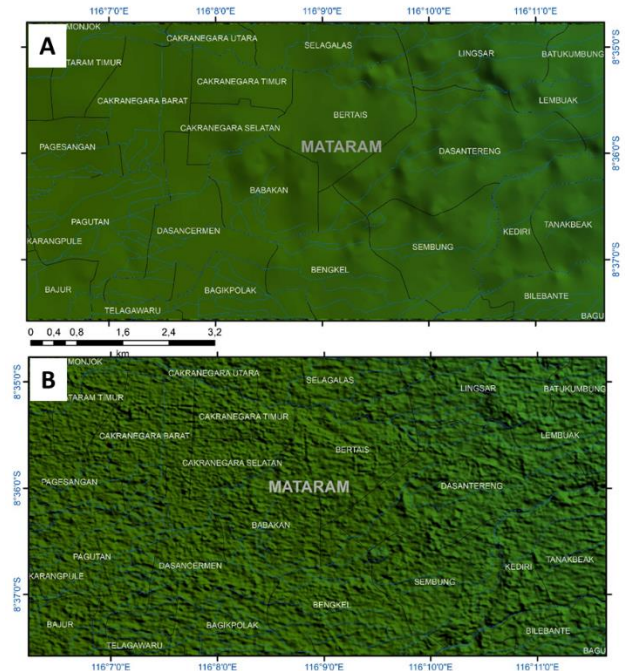
Figure 2. Comparison of DEM data derived from RBI contour map (A) and DEMNAS (B). As shows in the figure, DEMNAS data has more detailed morphology expression.
