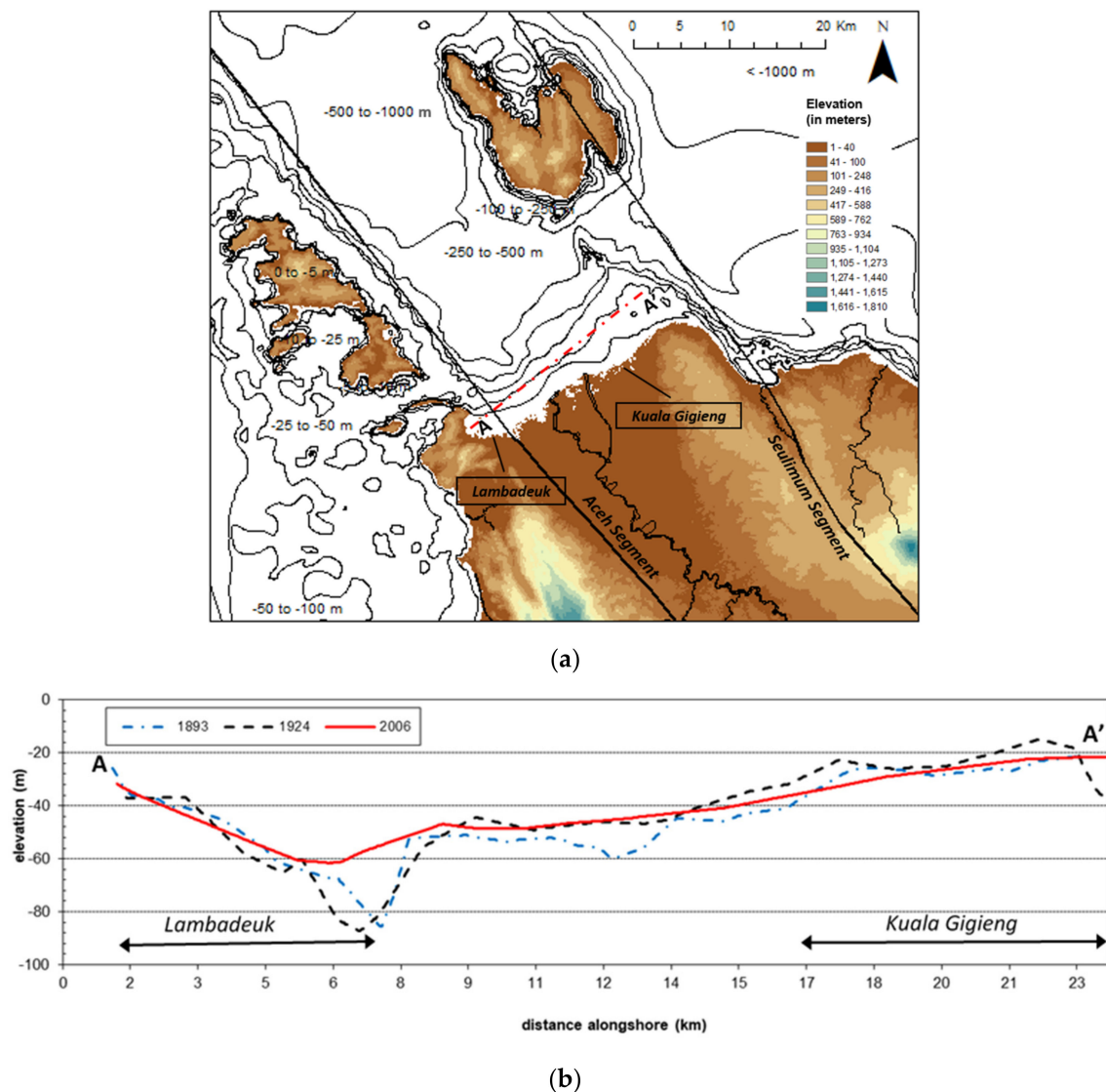
Figure 3. Banda Aceh is situated in the wedge between two tectonic fault segments of the Great Sumatran Fault System, i.e., the Aceh Segment on the southwest and Seulimum Segment on the northeast: (a) The map shows the topographic and bathymetric contours of the northern Sumatra region, and the two fault segments; (b) The multitemporal alongshore bathymetric profiles in front of Banda Aceh coast show higher elevation at Kuala Gigieng and lower down towards Lambadeuk. The bathymetric data of the year 1893 and 1924 was digitized from the Dutch Colonial Nautical Chart obtained from KITLV, and the 2006 bathymetry was obtained from the bathymetric survey conducted by UP-PSDA of Syiah Kuala University.
