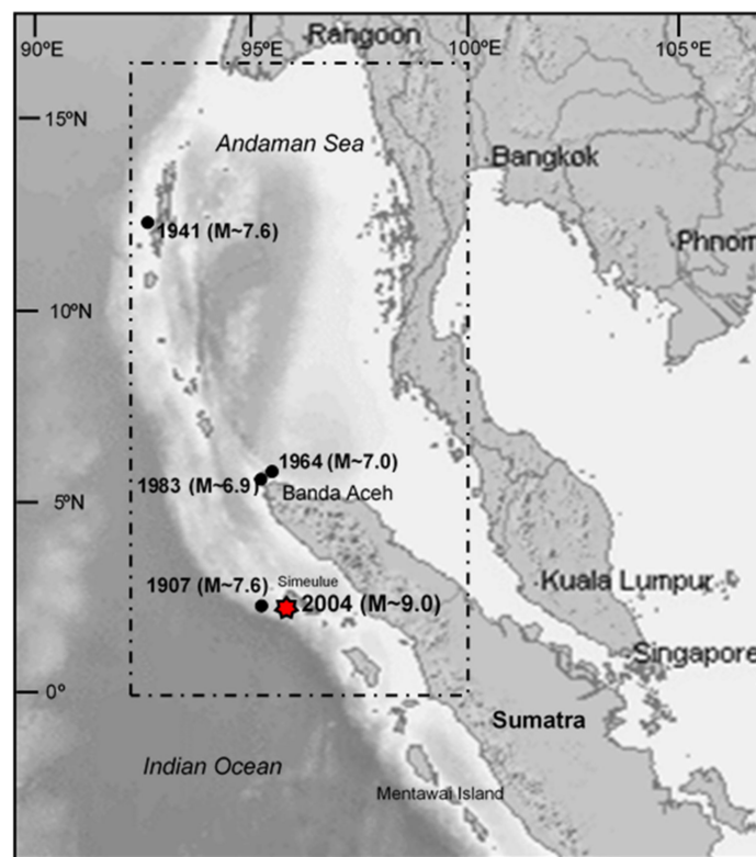
Figure 5. Regional earthquake occurrences at the northern Sumatra during the investigation period in the present study (1898–2017). The dashed-line rectangle shows the regional boundary of influence of the major ( M \geq 7.0 ) and moderate ( 6.5 \leq M < 7.0 ) earthquake records. Records of earthquakes M \geq 7.0 accompanied with the validity of tsunami occurrences are retrieved from the earthquake catalog by [54], and the tectonic earthquakes associated with the Great Sumatran Fault obtained from [55].
