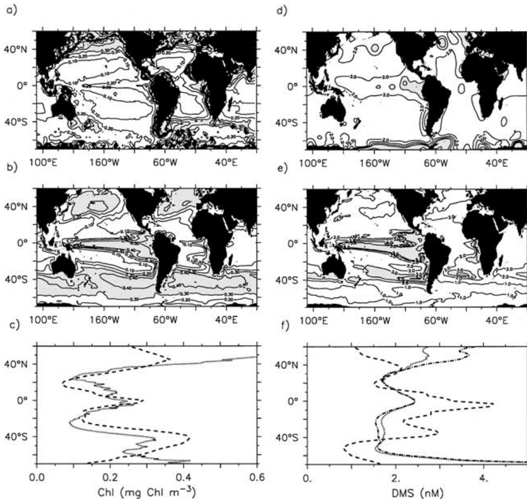
Fig. 1. Annual mean of surface chlorophyll (in \text{mg m}^{-3} ) (a) derived from remote sensing (SeaWiFS) and (b) from our control simulation. Isolines are every 0.1 \text{ mg Chl m}^{-3} . Shaded areas denote regions where chlorophyll is higher than 0.3 \text{ mg m}^{-3} . (c) Zonal means of simulated (dashed line) and satellite-derived (dotted line) surface chlorophyll distributions (in \text{mg m}^{-3} ). For the zonal mean of the satellite-derived chlorophyll, we have excluded coastal points. Annual mean of DMS concentration (in nM) at the sea-surface (d) from the climatology proposed by Kettle and Andreae (2000), and (e) from our control simulation. Isolines are every 1 from 0 to 5, every 5 from 5 to 30. Shaded areas denote regions where DMS is higher than 3 nM. (f) Zonal means of DMS concentrations predicted by the model (dashed line), and from the climatologies of Kettle et al. (1999) (dot-dashed line) and Kettle and Andreae (2000) (dotted line).
